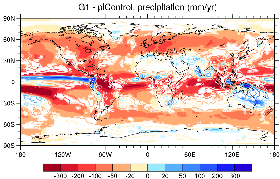
Fig. 8. Differences in precipitation between the simulations G1 and piControl in \text{mm yr}^{-1} , averaged over the four ESMs. In regions with continuous color shading all models agree in the sign of the response.
