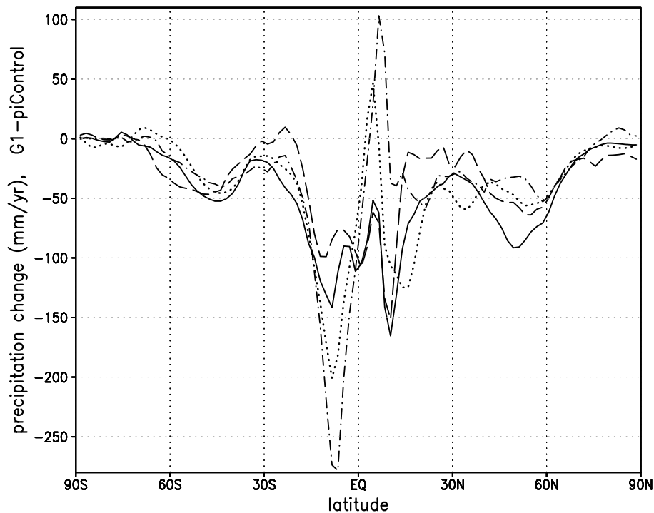
Fig. 7. Differences in zonally-averaged precipitation between the simulations G1 and piControl in \text{mm yr}^{-1} from the four ESMs. Solid: IPSL-CM5A, dashed: MPI-ESM, dotted: Nor-ESM, dot-dashed: HadGEM2-ES.
