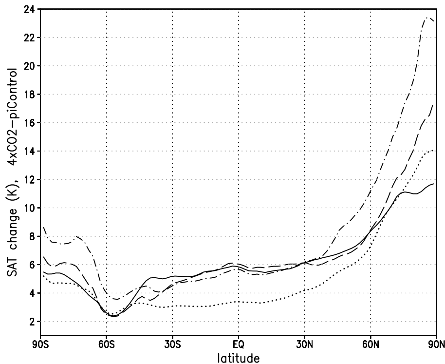
Fig. 11. Differences in zonally-averaged near surface air temperatures between the simulations abrupt4xCO 2 and piControl in K from the four ESMs. Solid: IPSL-CM5A, dashed: MPI-ESM, dotted: Nor-ESM, dot-dashed: HadGEM2-ES.
