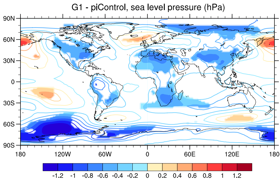
Fig. 6. Differences in sea level pressure between the simulations G1 and piControl in hPa, averaged over the four ESMs. In regions with continuous color shading all models agree in the sign of the response.
