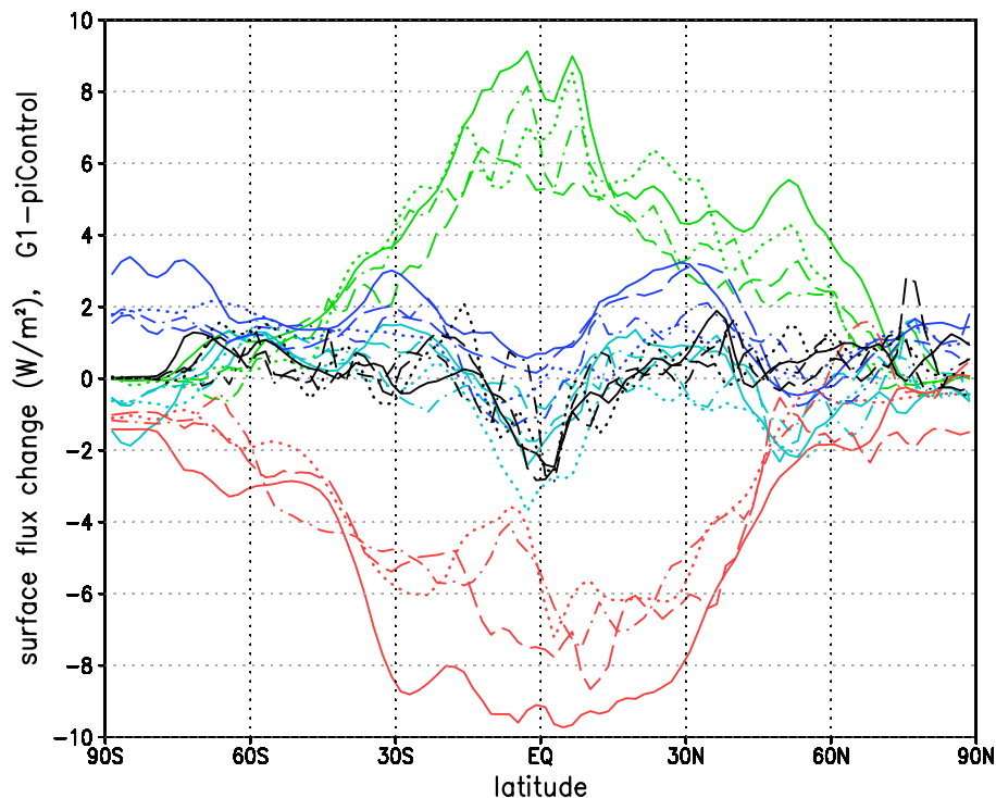
Fig. 2. Differences in zonally-averaged surface net downward energy fluxes between the simulations G1 and piControl in \text{Wm}^{-2} from the four ESMs. Solid: IPSL-CM5A, dashed: MPI-ESM, dotted: Nor-ESM, dot-dashed: HadGEM2-ES. Blue: longwave radiation, red: shortwave radiation, green: latent heat, cyan: sensible heat, black: sum of all four components. All fluxes are defined as positive in the downward direction.
