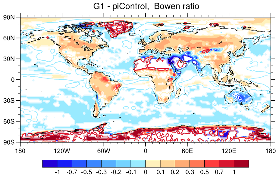
Fig. 9. Differences in Bowen ratio (ratio of surface sensible and latent heat fluxes) between the simulations G1 and piControl, averaged over the four ESMs. In regions with continuous color shading all models agree in the sign of the response.
