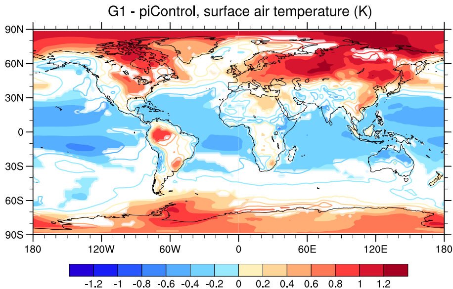
Fig. 5. Differences in near surface air temperatures between the simulations G1 and piControl in K, averaged over the four ESMs. In regions with continuous color shading all models agree in the sign of the response.
