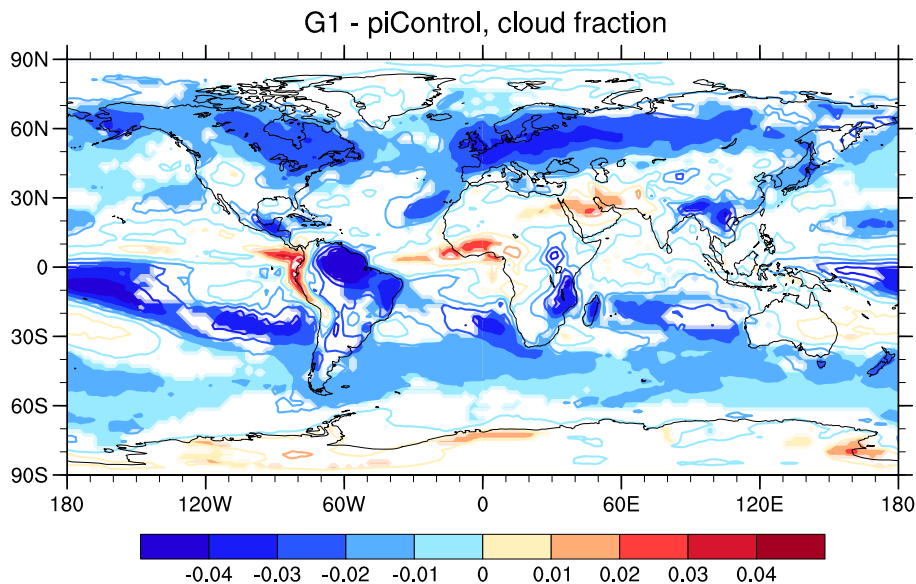
Fig. 10. Differences in total cloud fraction between the simulations G1 and piControl, averaged over the four ESMs. In regions with continuous color shading all models agree in the sign of the response.
