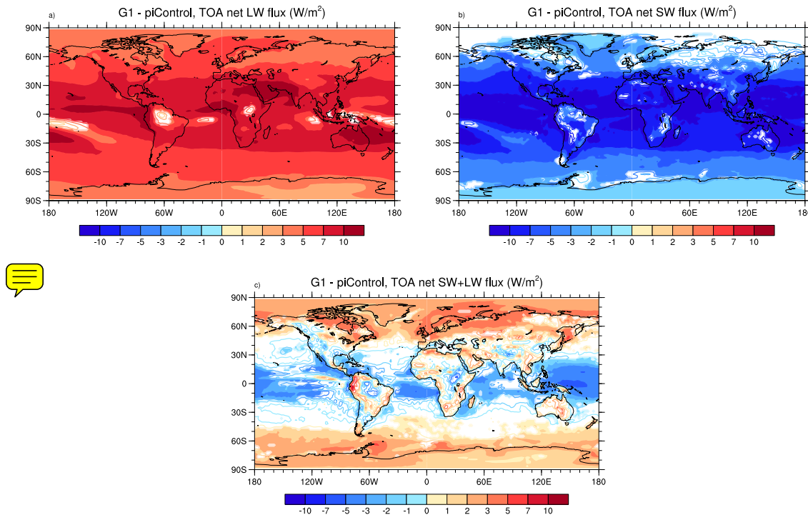
Fig. 1. Differences in TOA (top-of-atmosphere) net downward radiation fluxes between the simulations G1 and piControl in \text{Wm}^{-2} , averaged over the four ESMs. (a) Longwave (terrestrial), (b) shortwave (solar), (c) sum of long and short wave. In regions with continuous color shading all models agree in the sign of the response.
