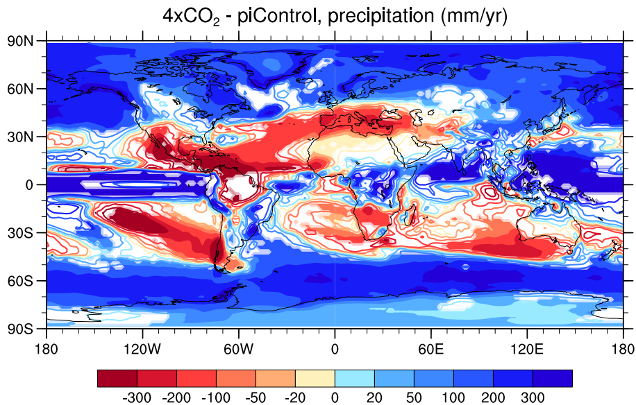
Fig. 12. Differences in precipitation between the simulations abrupt4xCO 2 and piControl in mm yr -1 , averaged over the four ESMs. In regions with continuous color shading all models agree in the sign of the response.
