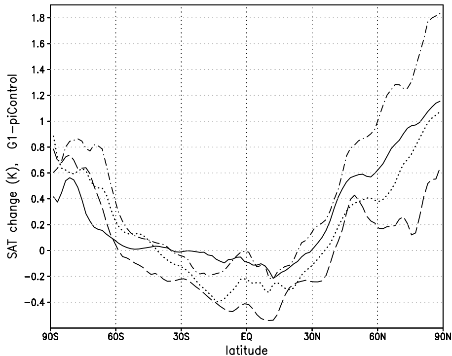
Fig. 4. Differences in zonally-averaged near surface air temperatures between the simulations G1 and piControl in K from the four ESMs. Solid: IPSL-CM5A, dashed: MPI-ESM, dotted: Nor-ESM, dot-dashed: HadGEM2-ES.
