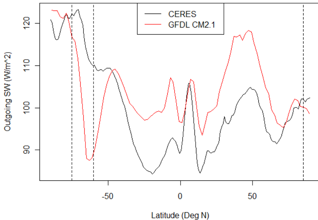
Fig. 2. All-sky outgoing SW flux by latitude
