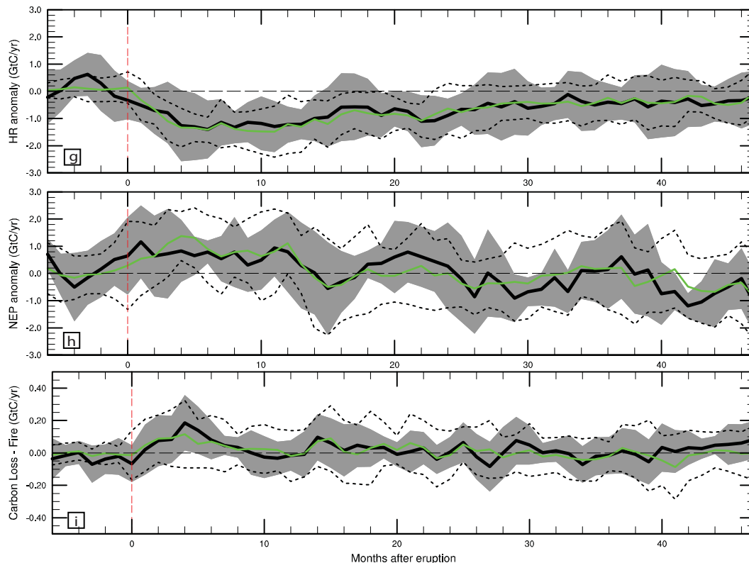
Fig. 8. Globally averaged (a–b) and integrated (c–f) monthly anomalies for the indicated variables, computed using both the “volcano-control” and “no-control” methods, averaged and composited for the 5 denoted eruptions in Table 1. Mean anomalies for each method are depicted with black and green lines, respectively, and the corresponding standard deviation is shown as a shaded area (“volcano-control”) and dotted lines (“no-control”). X-axis is months after eruption (dashed red line). Negative surface flux indicates uptake by land/ocean.
