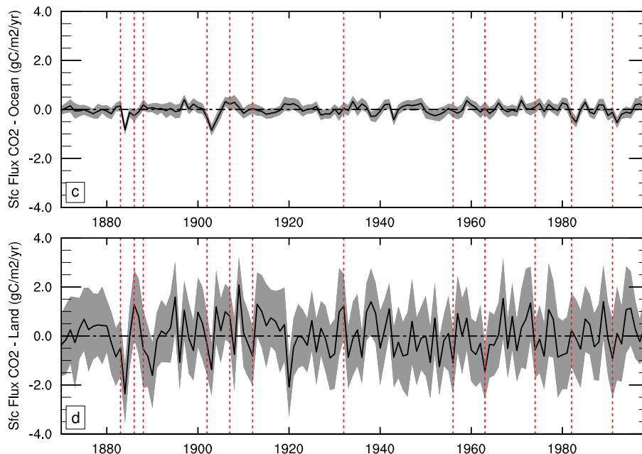
Fig. 1. Globally averaged yearly anomalies for surface temperature (a) , CO 2 (b) , surface flux of carbon to ocean (c) and land (d) from a coupled carbon-climate model, the CCSM3. The model included prescribed aerosol (volcanic, carbonaceous, and prognostic sulfate with corresponding emissions) and anthropogenic forcings. Shaded area indicates one standard deviation (computed from ensembles of paired runs) above and below anomaly, and dashed vertical red lines indicate years with eruptions from Table 1. Significant drops in surface temperature and flux of carbon to the land and ocean occur after multiple eruptions, while there is not as coherent of a signal in the atmospheric CO 2 record. While prescribed CO 2 is used for radiation in the model, the CO 2 in the runs plotted here is fully interactive.
