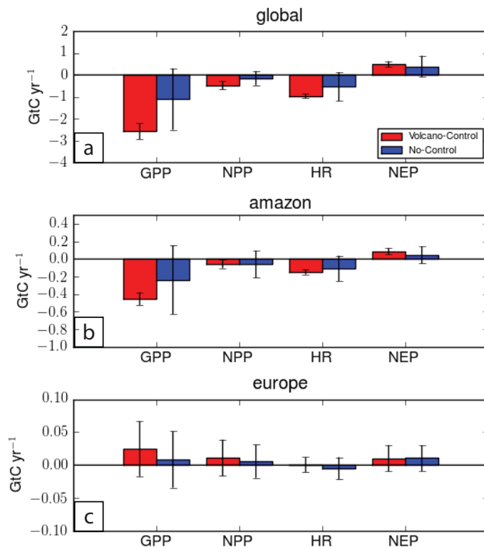
Fig. 10. Factors contributing to the net uptake of CO 2 from the atmosphere – gross primary production, net primary production, heterotrophic respiration, and net ecosystem productivity – totaled regionally and averaged across the subset of 5 eruptions in Table 1 for the two-year period immediately following the eruptions. Colored bars indicated mean anomalies for the indicated factor and region, and standard deviation of time-mean response computed at each gridpoint is plotted with error bars.
