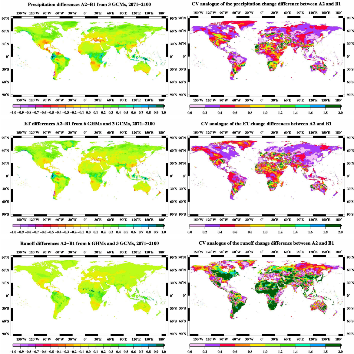
Figure S1: Absolute differences (mm/d; left column) and CV analogue (right column) of differences in the projected annual ensemble mean change between the A2 and B1 scenarios for precipitation from the 3 GCMs (upper row) as well as for evapotranspiration (middle row) and runoff (lower row) from 18 simulations (6 GHMs and 3 GCMs; note that only 6 GHMs were running B1) .
