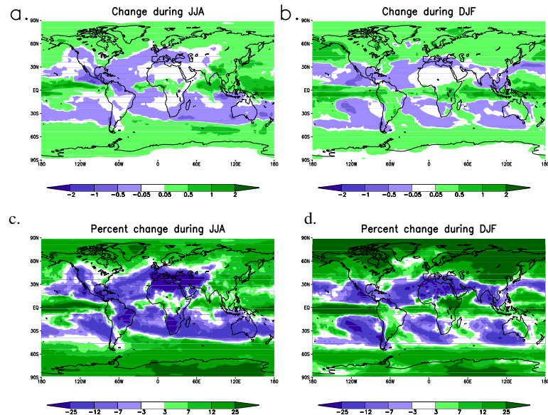
Fig. 11. IPCC model median change in precipitation ( \text{mm d}^{-1} ) from the 20th to 21st century for the northern summer (JJA) and winter (DJF) seasons: (a) Net change ( \text{mm day}^{-1} ) in June, July and August (JJA). (b) Net change ( \text{mm day}^{-1} ) in December, January and February (DJF). (c) Percentage change in JJA. (d) Percentage change in DJF. Note (i) the expansion of the subtropical dry zones, which coincides with reduced Amazon rainfall during northern summer, and (ii) the general strengthening of the ITCZ, which increases Amazon rainfall during the northern winter.
