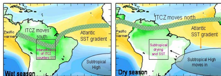
Fig. 13. A schematic diagram showing the two mechanisms under global warming (general subtropical drying, stronger Atlantic SST gradient and eastern Pacific warming) that may work in concert to produce a robust drier dry season in the southern Amazon and central Brazil (boxed area), but act in opposite directions in the Amazon wet season, leading to relatively small change. Background colors indicate climatological rainfall on land (green), the subtropical high pressure system (grey), and median IPCC model projected late 21st century SST with tropical mean removed (light brown and blue).
