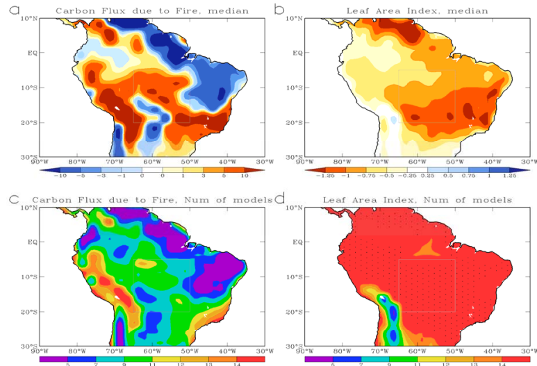
Fig. 9. Annual changes of ecosystem variables from the 20th Century (1961–1990) to the 21st Century (2070–2099) for (a) Carbon release due to fire ( \text{g m}^{-2} \text{y}^{-1} ), (b) LAI, from the median of the VEGAS model driven by the 15 IPCC models; and the number of models that project (c) an increase in fire, (d) a decrease in LAI (all 15 models show decrease in the dotted regions).
