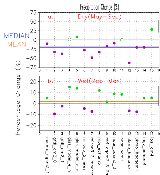
Fig. 7. Individual model precipitation change from the 20th to 21st century averaged over the SAB region for the dry season (a) and wet season (b). The majority of models suggest a drying of the dry season. The median of these models is shown by the blue line, and the mean in orange. Green dots denote an increase in precipitation, purple dots a decline. Models suggesting a change close to zero have open circles.
