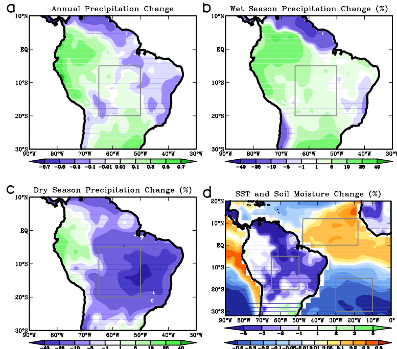
Fig. 2. Future changes in the Amazon and surrounding regions according to the median of 15 IPCC models calculated by taking the difference between the mean of the period of 2070–2099 and that of 1961–1990 for: (a) Annual mean precipitation ( \text{mm d}^{-1} ); (b) Wet season precipitation (%); (c) Dry season precipitation (%); (d) Annual sea surface temperature ( ^{\circ}\text{C} ) with its tropical mean removed and annual mean soil moisture (%).
