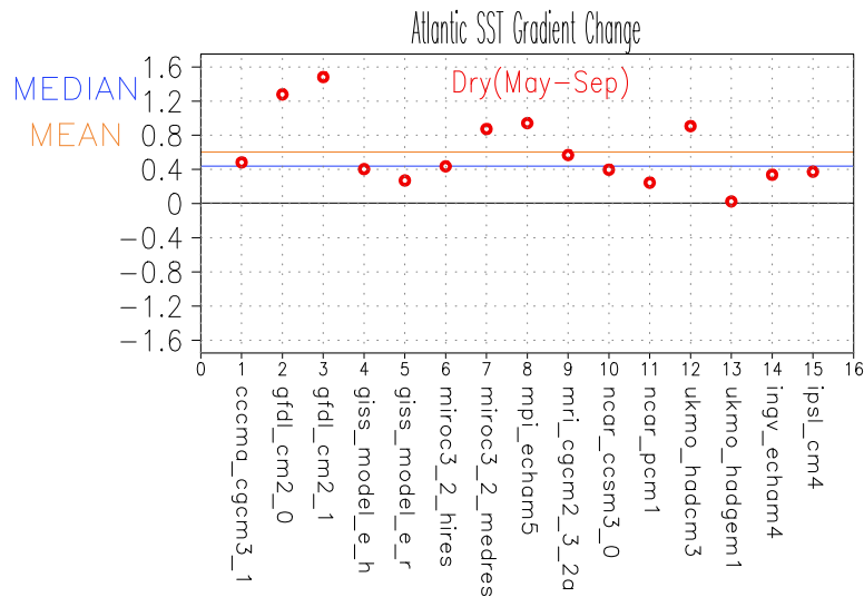
Fig. 10. Individual model results for change in the Atlantic SST gradient over the next century for the dry season (May–September). The North Atlantic is defined as ( 15^{\circ}\text{S} – 30^{\circ}\text{S} , 10^{\circ}\text{W} – 30^{\circ}\text{W} ), the south is defined as ( 15^{\circ}\text{S} – 30^{\circ}\text{S} , 10^{\circ}\text{W} – 30^{\circ}\text{W} ). The boxes can be viewed on Fig. 2d. The North–South SST gradient increases for all models. The median change in temperature gradient is shown in blue, and mean in orange.
