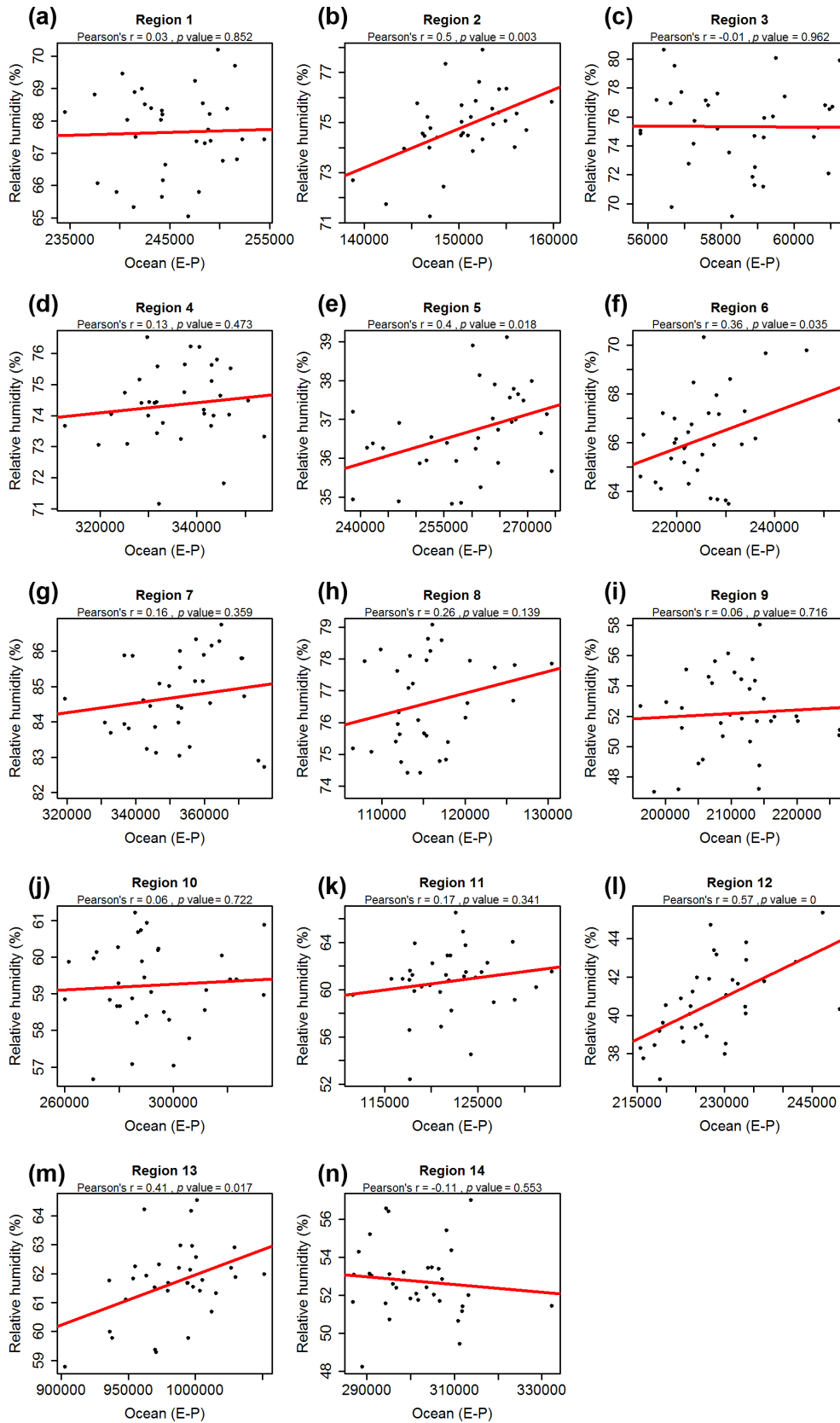
Figure 8. Relationships between the annual oceanic contribution to annual precipitation ( E-P ) and the annual RH in the target regions.
