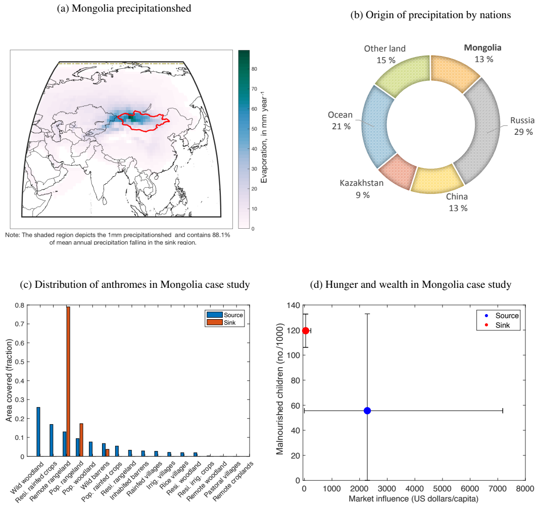
Figure 2. Mongolia case study including (a) precipitationshed analysis, (b) key source countries, (c) comparison of land uses between the country and its precipitationshed, and (d) comparison of economic and food security aspects of country and source regions.
