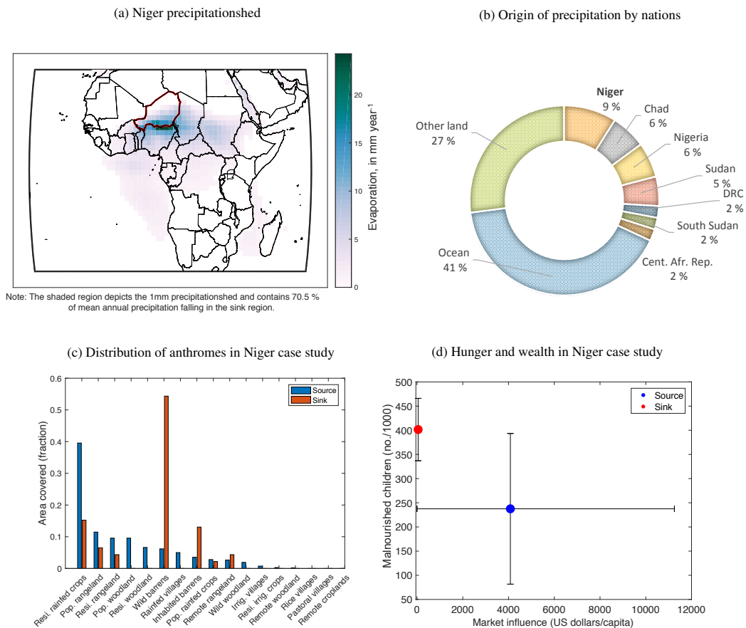
Figure 3. Niger case study including (a) precipitation shed analysis, (b) key source countries, (c) comparison of land-uses between the country and its precipitation shed, and (d) comparison of economic and food security aspects of country and source regions.
