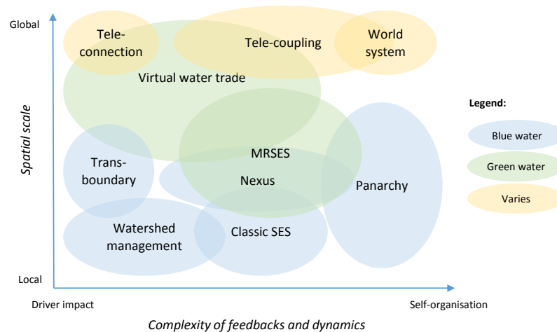
Figure 6. Concept of MRSES in relation to other concepts pertinent to human–water system research along the axes of spatial scale and feedback complexity considered and in terms of water flows considered. Blue water refers to liquid water in rivers, lakes, and aquifers, whereas green water here refers to terrestrial evaporation and moisture flows.
