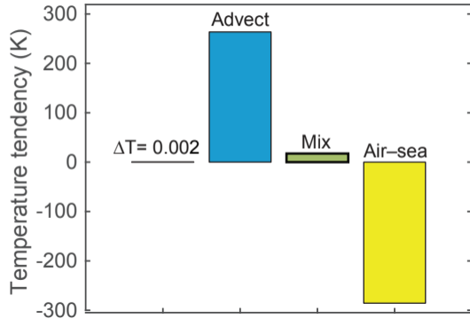
(a) Preindustrial control; 0–100 m
