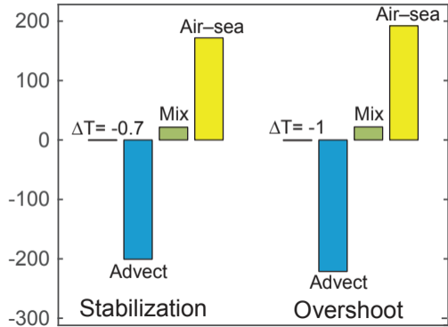
(b) Perturbation - preindustrial control; 0–100 m
