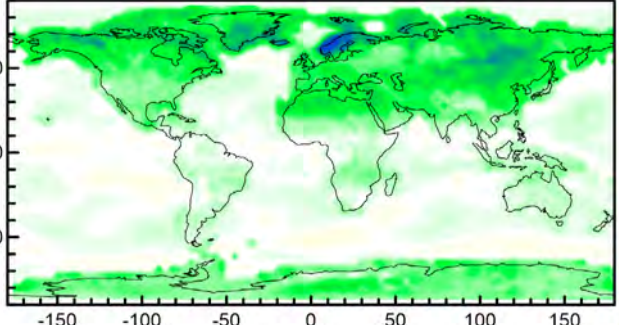
(b) Northward wind (850 hPa) link to eastward OGW drag (10 hPa)
