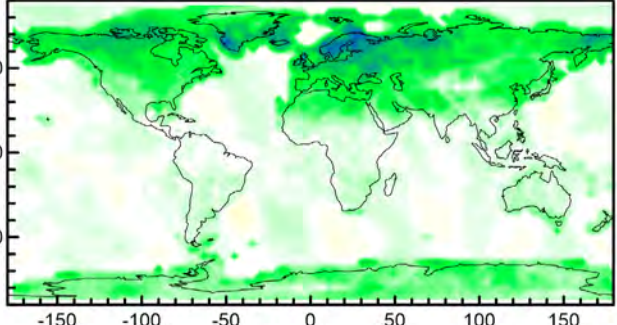
Northward OGW drag (10 hPa): fraction of variance explained
