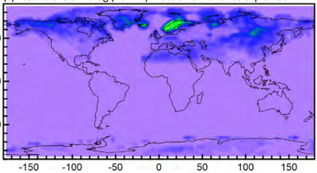
(c) Eastward OGW drag (10 hPa): fraction of variance explained
