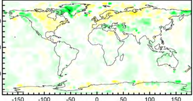
(c) Eastward OGW drag (10 hPa): fraction of variance explained
