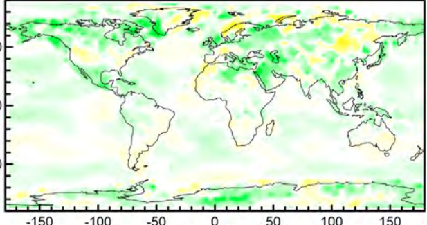
Northward wind (850 hPa) link to northward OGW drag (10 hPa)
