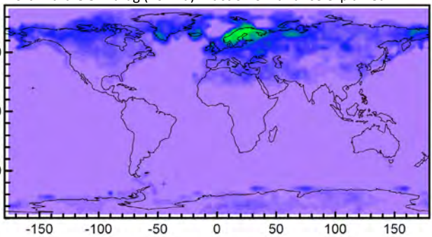
Northward OGW drag (10 hPa): fraction of variance explained
