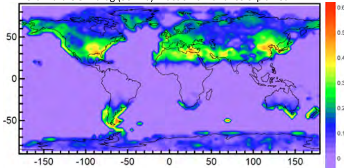
Northward OGW drag (50 hPa): fraction of variance explained
