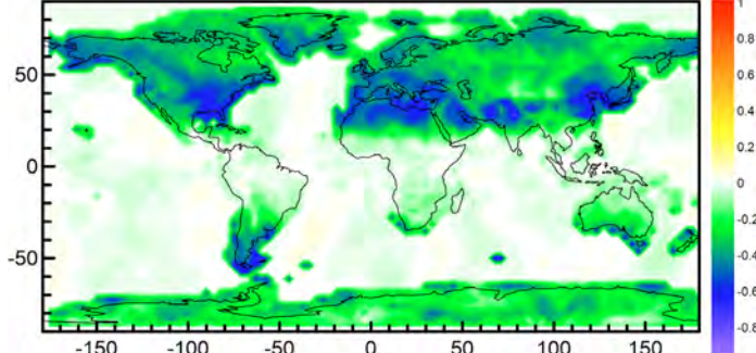
Northward OGW drag (50 hPa): fraction of variance explained
