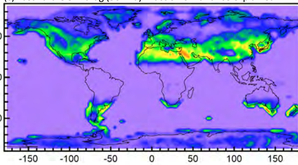
(c) Eastward OGW drag (50 hPa): fraction of variance explained
