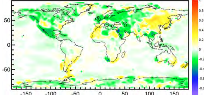
Northward wind (850 hPa) link to northward OGW drag (50 hPa)
