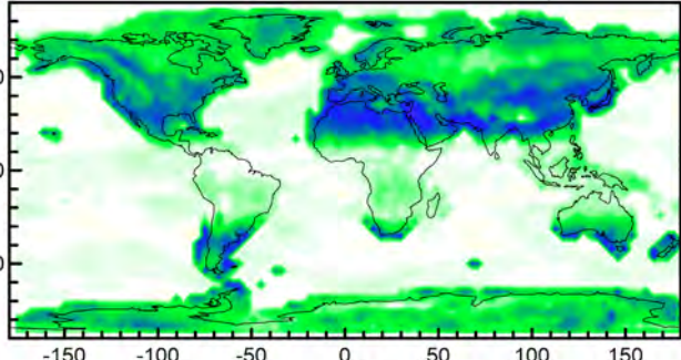
(b) Northward wind (850 hPa) link to eastward OGW drag (50 hPa)
