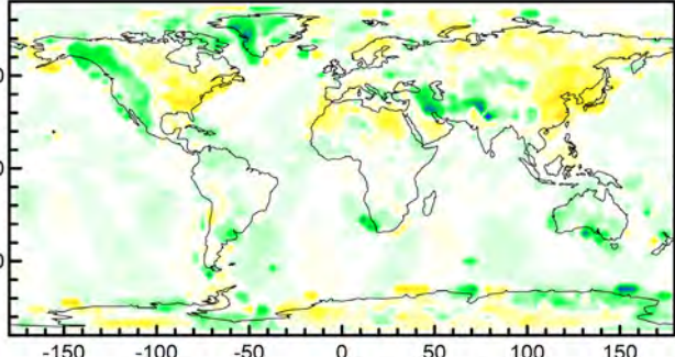
(c) Eastward OGW drag (50 hPa): fraction of variance explained
