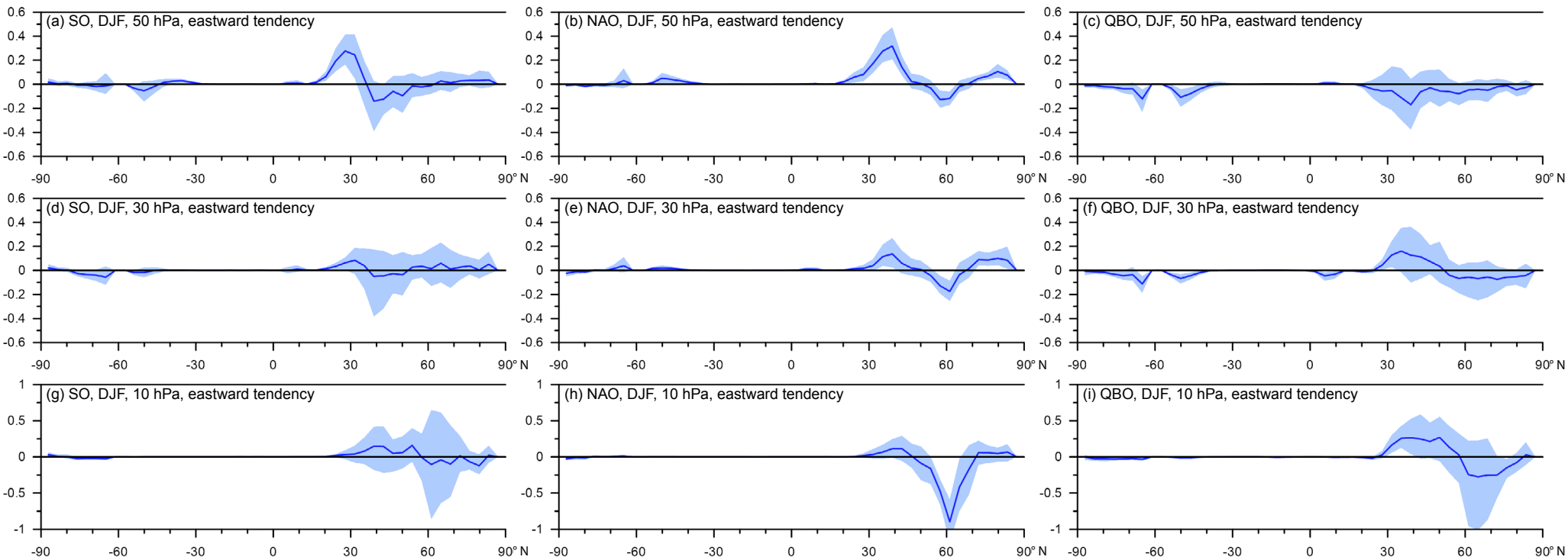
Regression-estimated OGWD responses ( \text{m s}^{-1} \text{ day}^{-1} ) to indices of SO, NAO and QBO and their 95 % confidence interval
