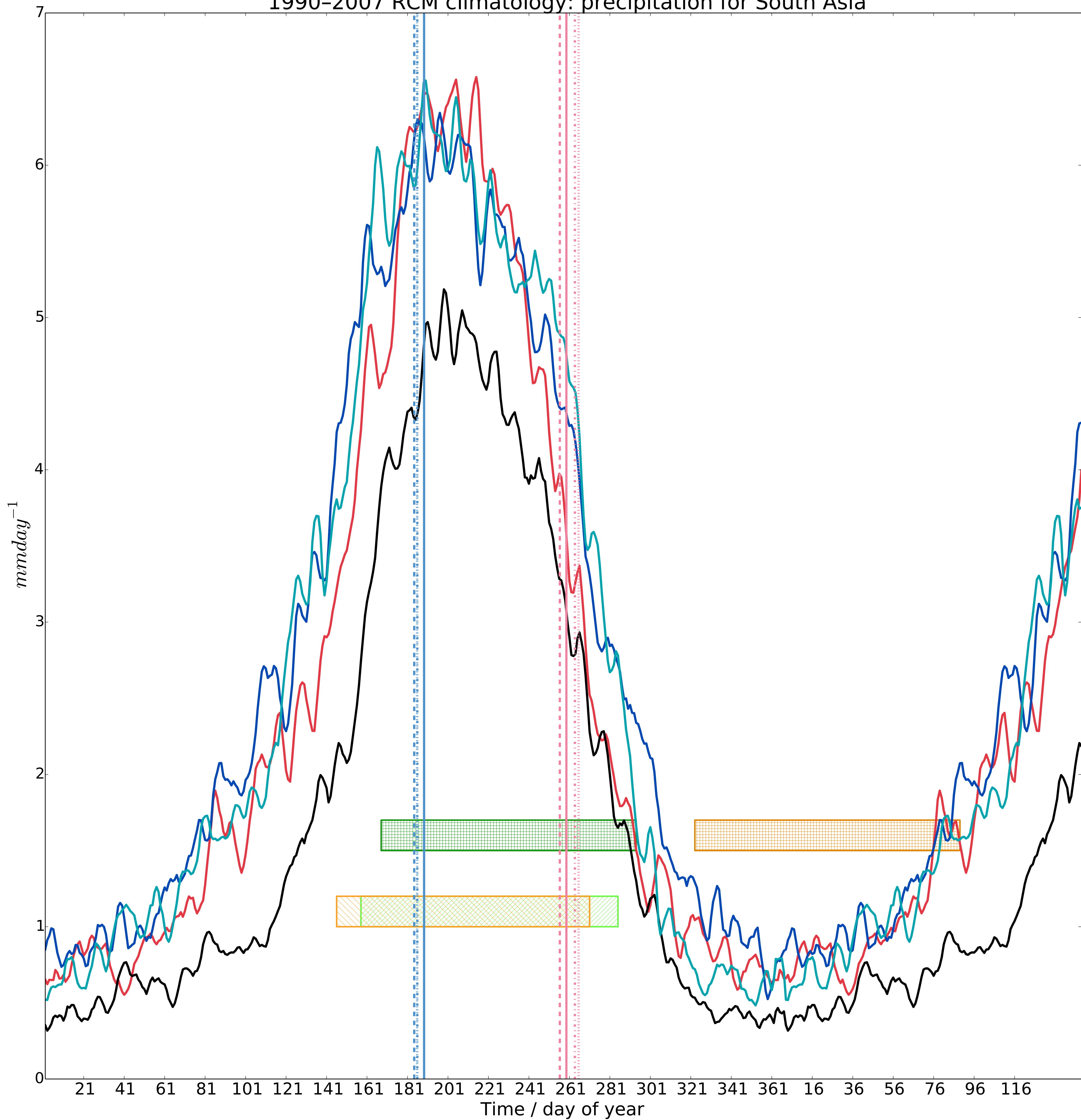
1990-2007 RCM climatology: precipitation for South Asia
