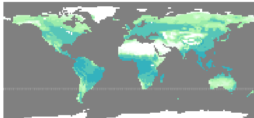
(b) PI vegetation cover
