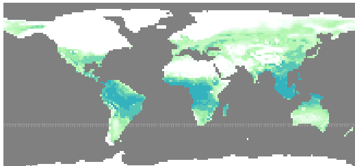
(a) LGM vegetation cover
