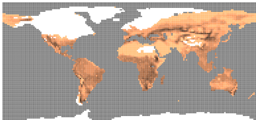
(c) LGM carbon storage
