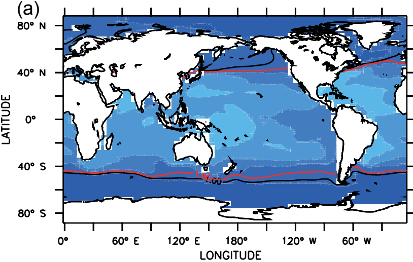
RCP8.5_AOA_G
