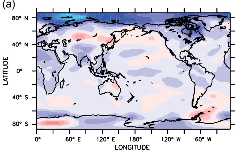
RCP8.5_AOA_G
