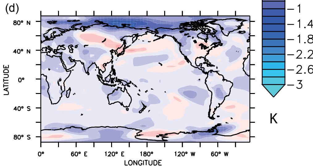
RCP8.5_AOA_T
