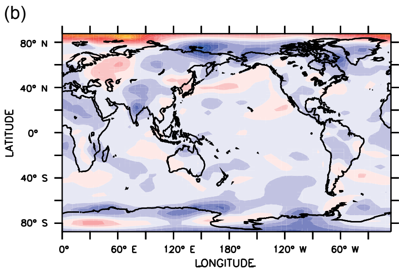
RCP8.5_AOA_SP
