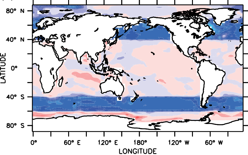
RCP8.5_AOA_SP
