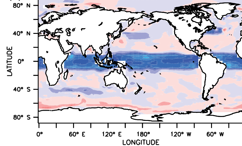
RCP8.5_AOA_T
