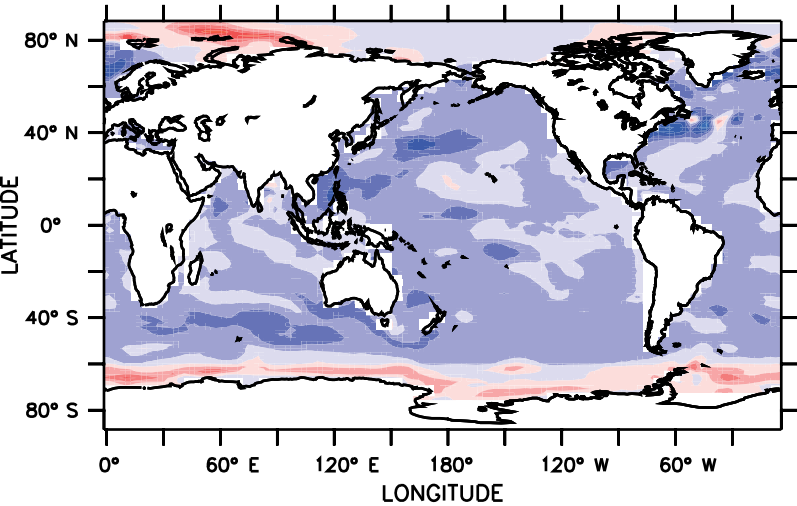
RCP8.5_AOA_G
