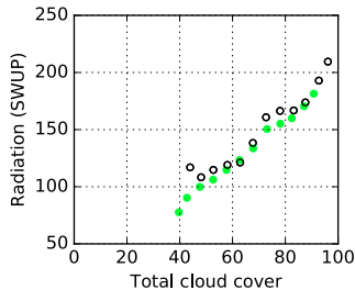
EC-EARTH EC-EARTH3
