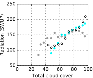
CNRM-CM5 CNRM-AM-PRE6
