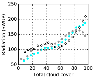
CNRM-CM5 CNRM-AM-PRE6
