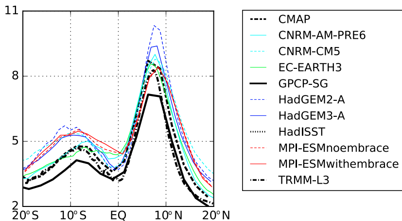
Precipitation (mm day -1 )
