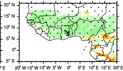
(f) Mix2 minus GPCP (%)
