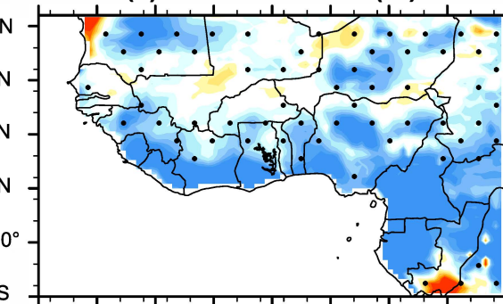
(b) Mix1 minus CRU ( ^{\circ}\text{C} )
