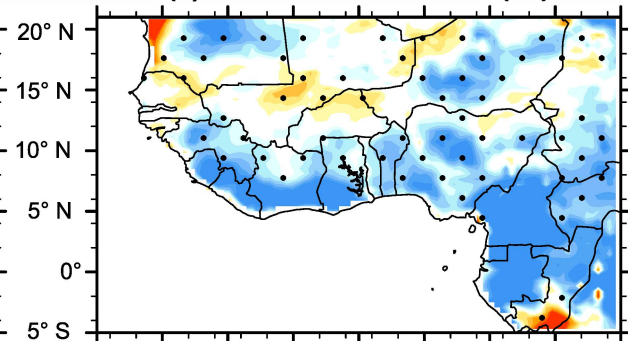
(c) Emanuel minus CRU ( ^{\circ}\text{C} )
