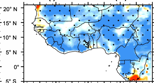
(f) Mix2 minus CRU ( ^{\circ}\text{C} )
