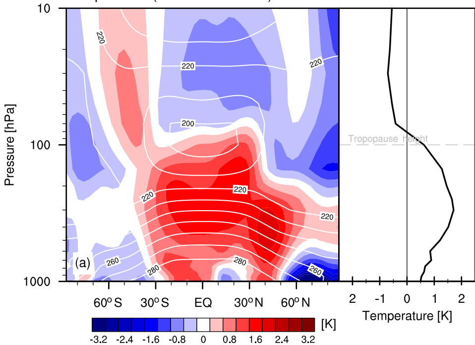
Temperature (RETRO - CNTRL)
