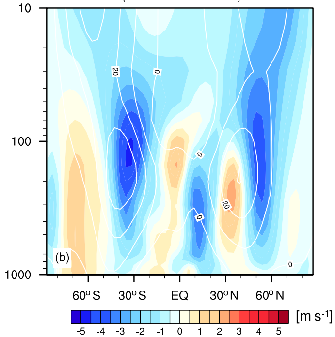
Zonal wind (RETRO + CNTRL)
