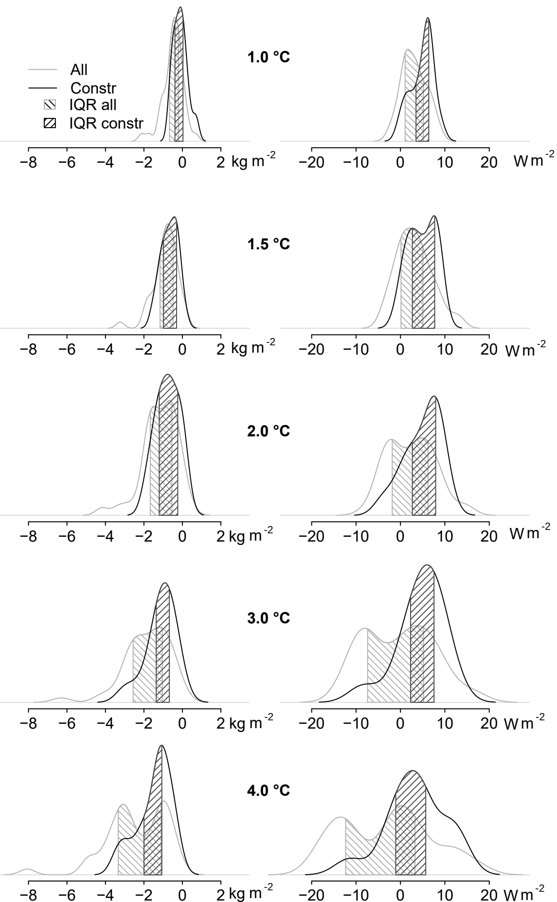
(a) \Delta\text{top SM}
