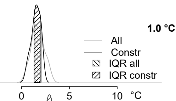
(a) \Delta T X_x
