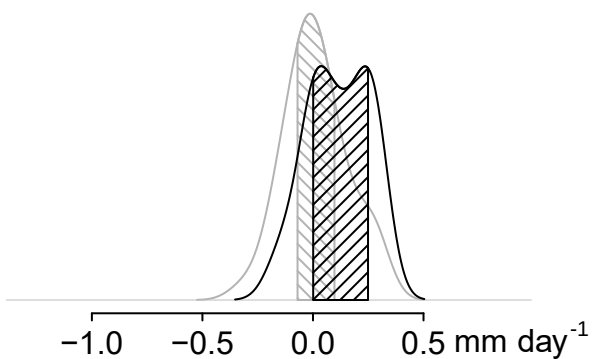
(b) \Delta \text{precip}
