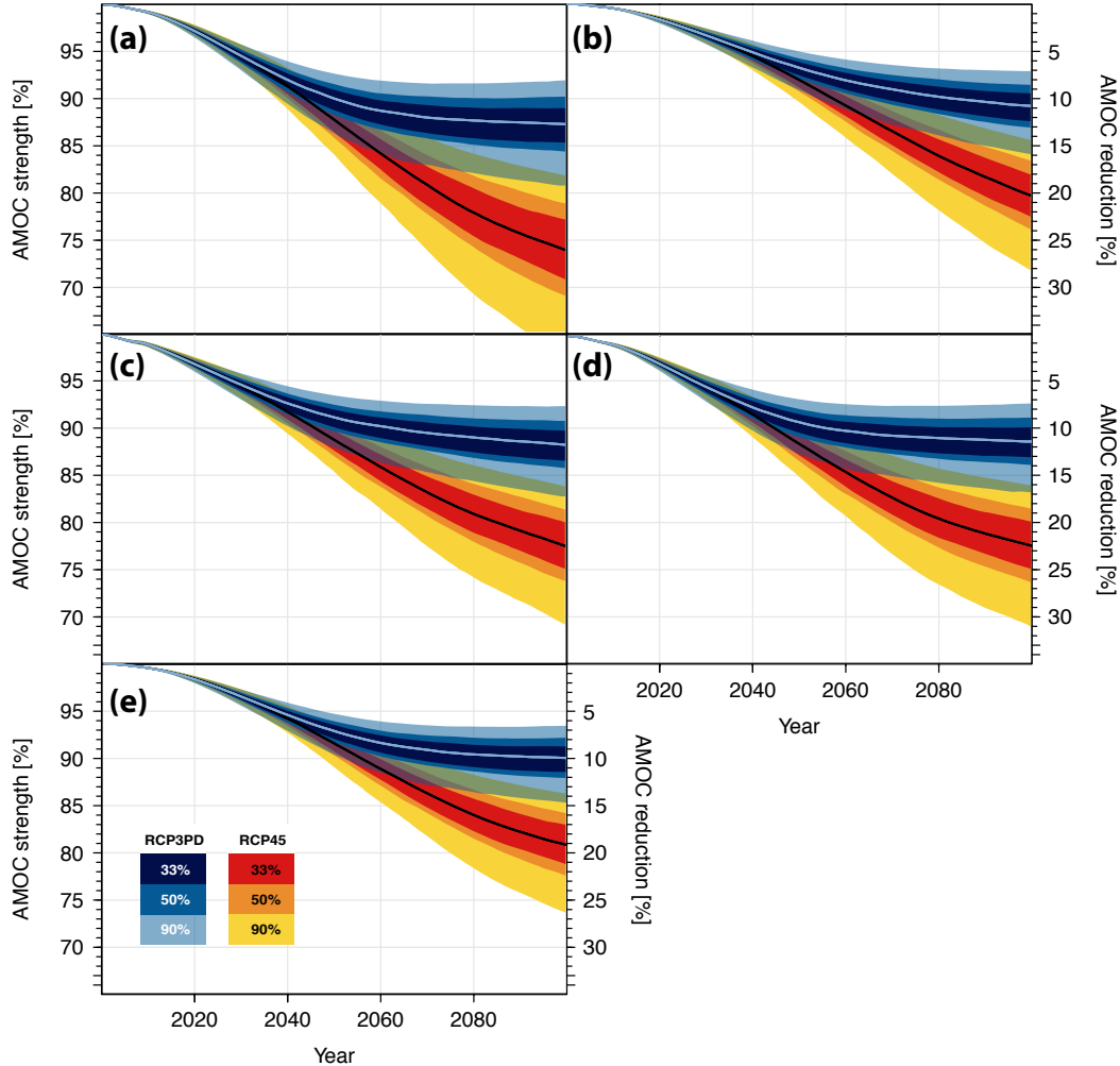
Figure S1. The projected AMOC weakening as in Fig. 4 of the manuscript for each ensemble member separately: (a) GFDL_R30, (b) MRI_CGCM_2.3, (c) MPI_ECHAM5, (d) MIROC3.2, (e) NCAR_CCSM2.0.
