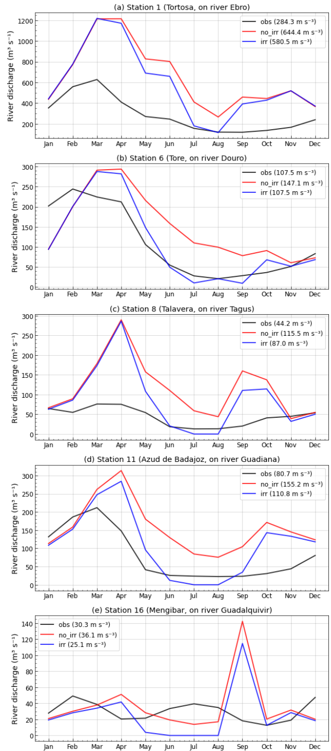
Figure 5. Impacts of irrigation on river discharge. Mean seasonal cycle of river discharge ( \text{m}^3 \text{ s}^{-1} ) in observations (black) and the no_irr (red) and irr (blue) simulations at five stations: (a) Tortosa (Ebro), (b) Tore (Douro), (c) Talavera (Tagus), (d) Azud de Badajoz (Guadiana), and (e) Mengibar (Guadalquivir). Annual mean values are shown in the legend. A mask is applied to the simulations to filter out months without corresponding observation data.
