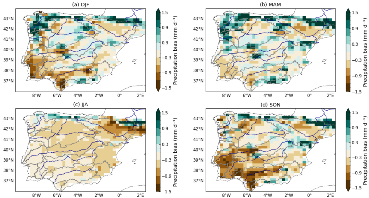
Figure D1. Seasonal mean biases of precipitation ( \text{mm d}^{-1} ) in the no_irr simulation compared with the GPCC product (2010–2019).
