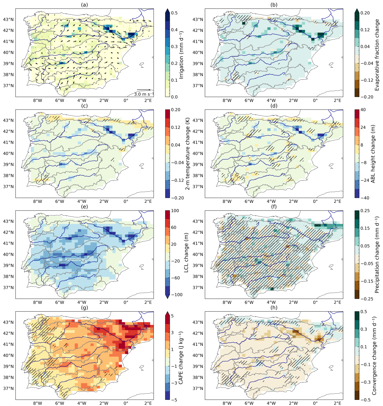
Figure G3. Autumn irrigation and its impacts (SON, 2010–2022). (a) Irrigation ( \text{mm d}^{-1} ) and 10 m wind ( \text{irr} simulation). Mean changes in the presence of irrigation ( \text{irr} - \text{no\_irr} ): (b) evaporative fraction, (c) 2 m temperature (K), (d) atmospheric boundary layer height (m), (e) lifting condensation level (m), (f) precipitation ( \text{mm d}^{-1} ), (g) convective available potential energy ( \text{J kg}^{-1} ), (h) moisture convergence ( \text{mm d}^{-1} ). Hatching indicates areas where the change is not statistically significant.
