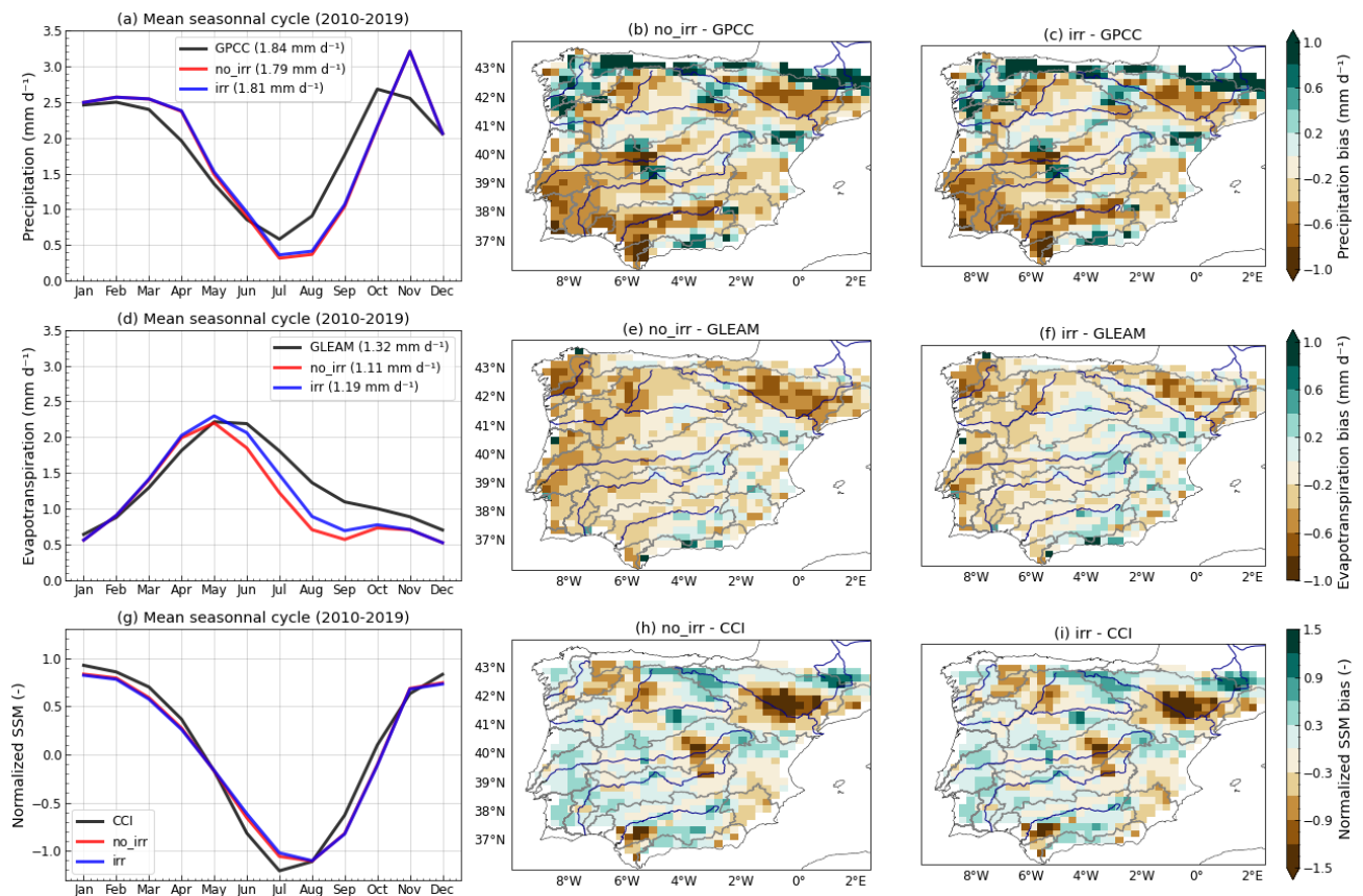
Figure 6. Evaluation of simulated precipitation ( P ) and evapotranspiration ( ET ) over the Iberian Peninsula continental subdomain, from 2010 to 2019. (a) Mean seasonal cycle of P ( \text{mm d}^{-1} ) for the two simulations and GPCC product (annual mean values are shown in the legend), annual mean P bias of the (b) no_irr and (c) irr simulations relative to the GPCC product ( \text{mm d}^{-1} ). (d) Mean seasonal cycle of ET ( \text{mm d}^{-1} ) for the two simulations and GLEAM4 product (annual mean values are shown in the legend), annual mean ET bias of the (e) no_irr and (f) irr simulations relative to the GLEAM4 product ( \text{mm d}^{-1} ). (g) Mean seasonal cycle of normalized SSM for the two simulations and CCI product, annual mean normalized SSM bias of the (h) no_irr and (i) irr simulations relative to the CCI product.
