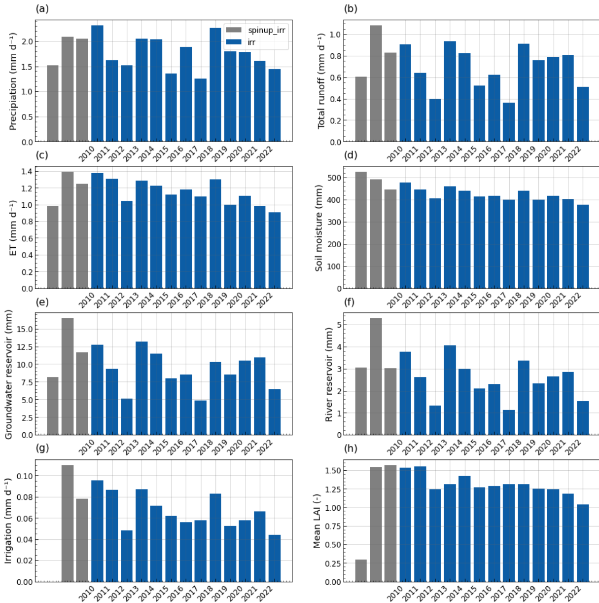
Figure B1. Annual mean values over the Iberian Peninsula in the 3-year spin-up and irr simulation for (a) precipitation, (b) total runoff, (c) evapotranspiration, (d) soil moisture in the 2 m soil column, (e) groundwater reservoir, (f) river reservoir, (g) irrigation, (h) mean Leaf Area Index. Annual values are very similar for the no_irr simulation but irr was used to include irrigation.
