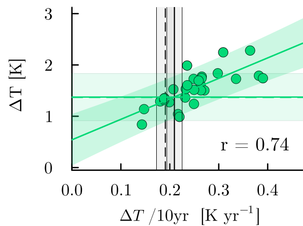
ssp126, 2030
