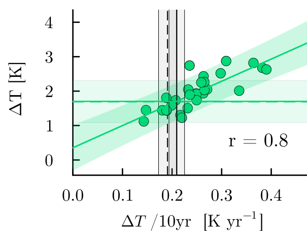
ssp126, 2090
