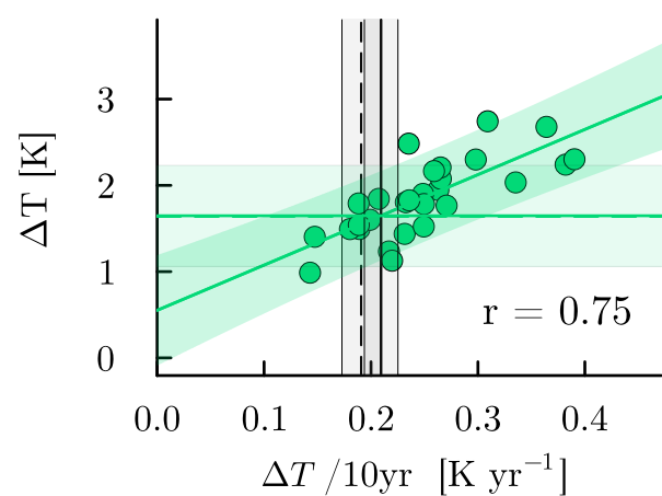
ssp126, 2050
