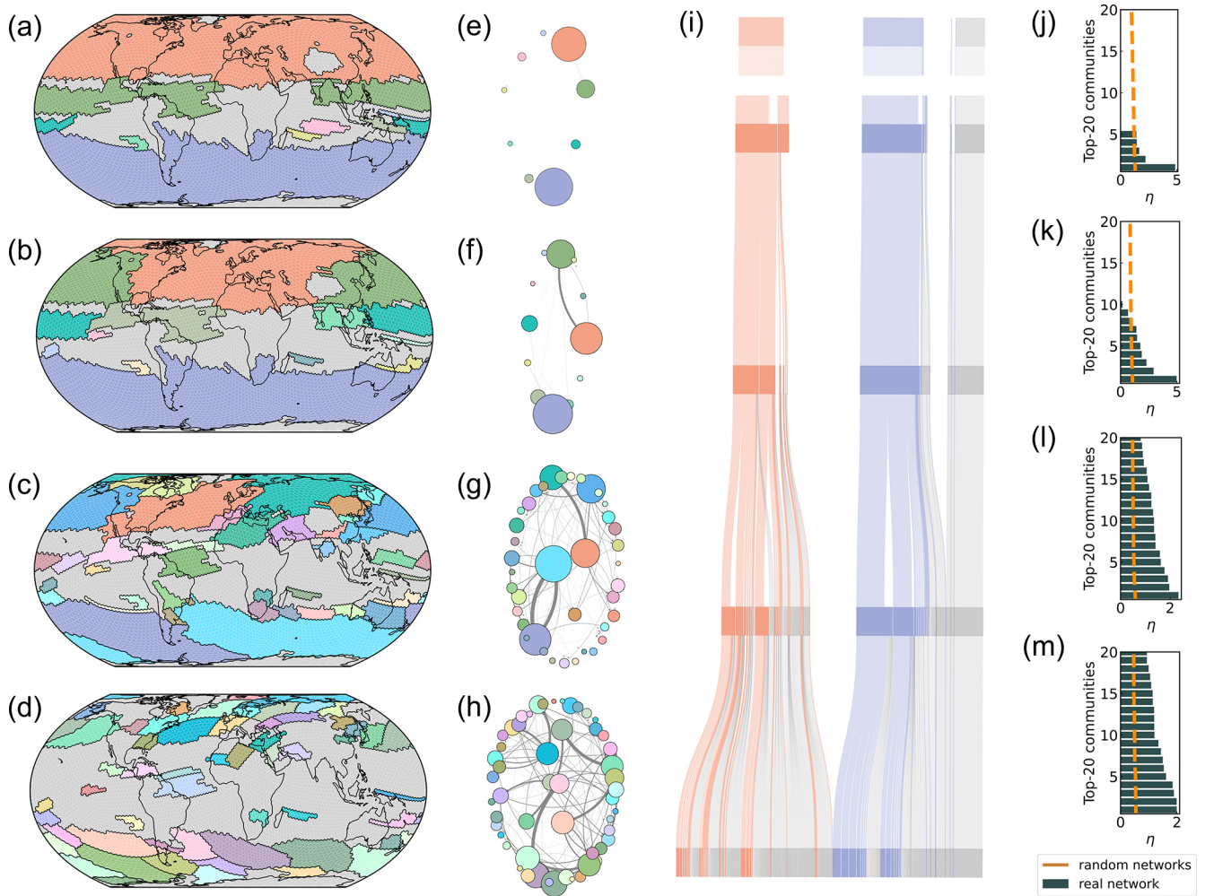
Figure 6. The hierarchical organization of AR basins as identified through Infomap community detection. Communities are arranged hierarchically from top to bottom across each column. Panels (a)–(d) show the communities from level-1 to level-4 (discarding level-0). Small communities ( < 15 grid cells) are absorbed into the grey background. Panels (e)–(h) display intra- and inter-community flows in a network representation where each node represents a community at the given level. Node size scales with total flow, edge width scales with inter-community flow. (i) Sankey diagram to visualize hierarchical branching of communities into smaller and smaller sub-communities. Each vertical box represents a separate community, colored by its parent community at level-0 (indicated at the top with gap below). Each connection represents how a community is split into sub-communities, with grey boxes/connections denoting discarded small communities. Panels (j)–(m) evaluate the quality of the top-20 highest flow communities at each level in terms of their flow ratio \eta , i.e., the ratio from intra- to inter-community flows. These are compared to the 95 %-quantile from realizations of the FRW network model.
