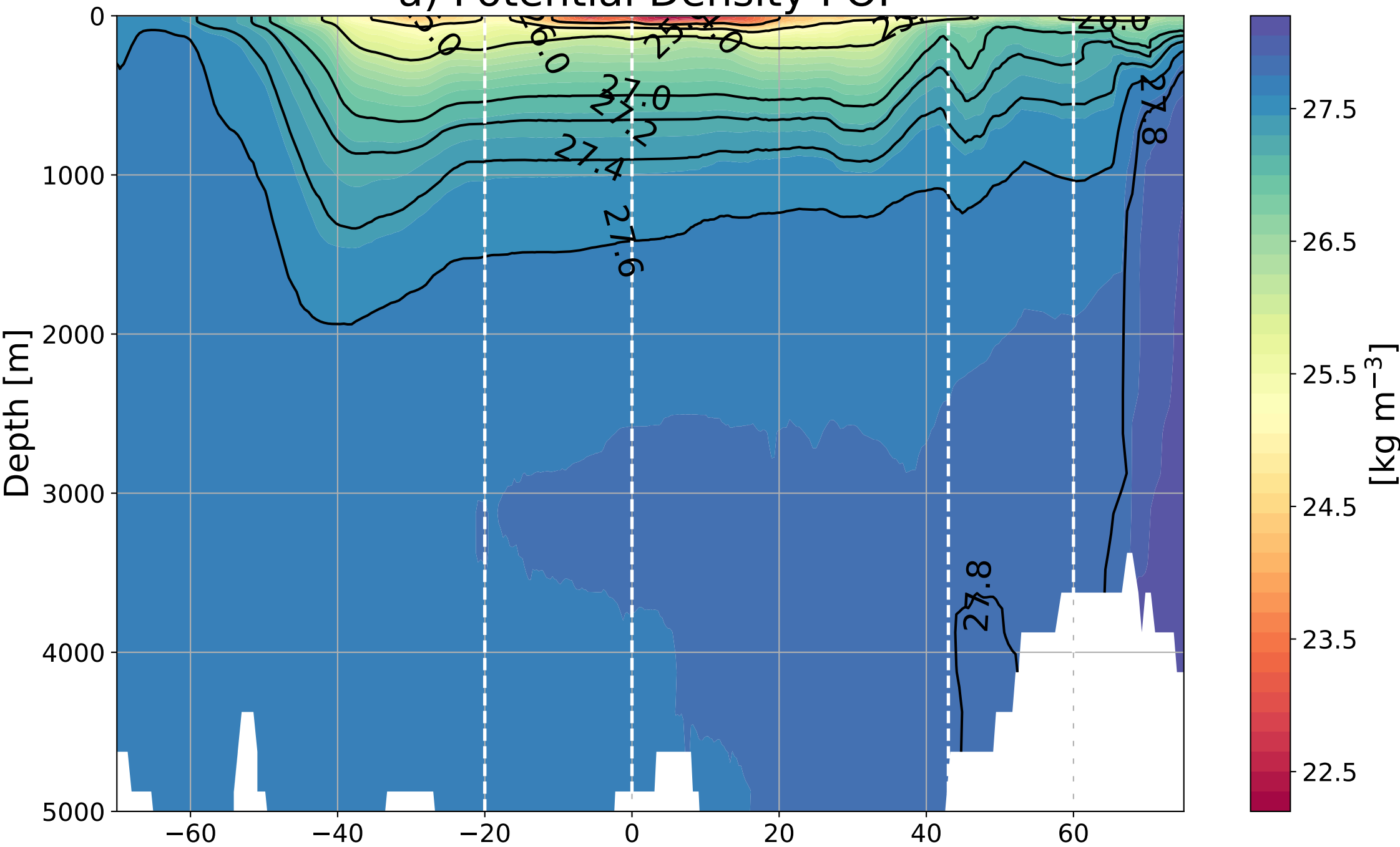
a) Potential Density POP
