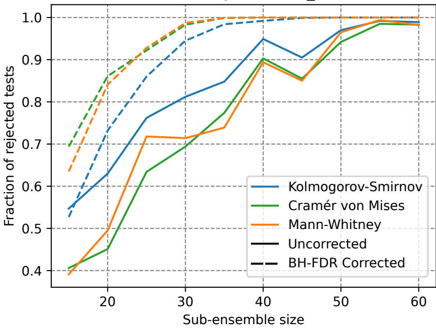
5% change in clubb_c1
