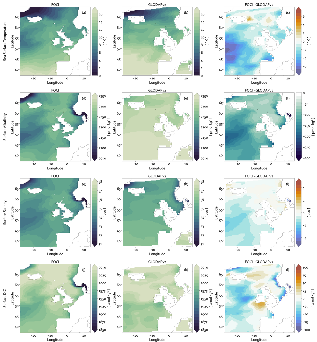
Figure 2. Comparison of FOCI-MOPS mean fields (1972–2013) and 2021 GLODAPv2 observations, along with their differences, for sea surface temperature (a, b, c), surface alkalinity (d, e, f), surface salinity (g, h, i), and surface DIC (j, k, l).
