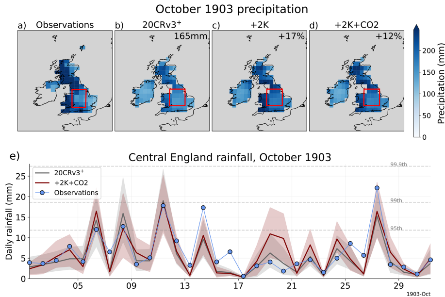
Figure 8. October rainfall in (a) observations (HadUKGrid at 60km resolution (Hollis et al., 2019)) and (b–d) the reanalysis experiments. The value in the top right of panel (b) is the average rainfall over the UK and Ireland in 20CRv3 + . The corresponding increase compared to 20CRv3 + is shown in the top right of panels (c) and (d). Panel (e) shows daily rainfall over Central England (the red boxed region, also used in Fig. 2; using reanalysis data from 09:00–09:00 UTC to match the observational definition). Shading shows the 10 %–90 % range across the ensemble and grey dashed lines indicate all-year daily rainfall percentiles in 20CRv3 + for 1903. Note that the boxes used to define the Central England region differ by a small amount in the observations compared to the reanalyses due to differences in the grids used (cf. the boxes in panels a and b).
