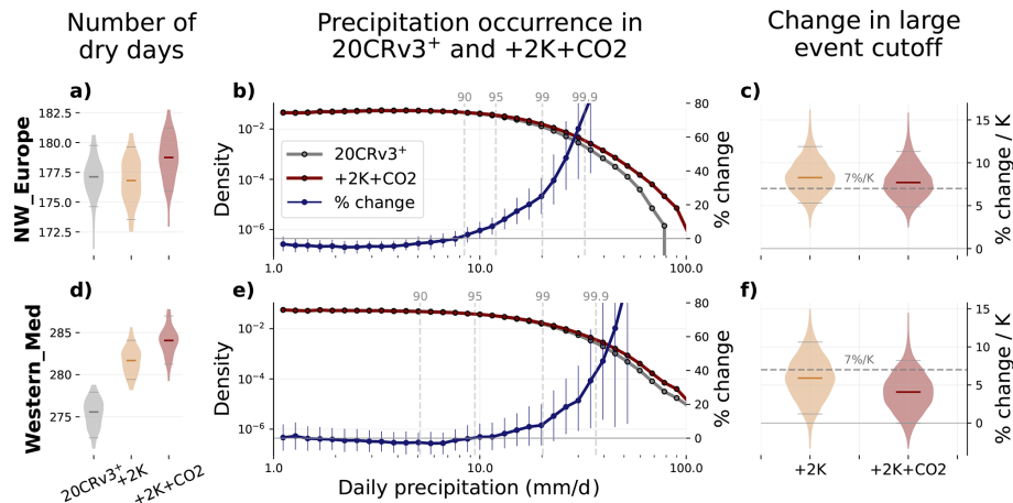
Figure 7. Precipitation characteristics of the NW_Europe (a–c) and Western_Med (d–f) regions. (a, d) Number of dry days, defined as days experiencing less than 1 mm of rain (here 1.04 mm due to numerical rounding). The median is shown by the horizontal line and the violin shows the distribution of ensemble members. (b, e) Daily precipitation occurrence in 20CRv3 + and +2 K + CO 2 . The blue line shows the percentage change in each bin in +2 K + CO 2 . Error bars show the 10%–90 % range through sampling all combinations of ensemble members, and vertical dashed lines show percentiles of the precipitation distribution in 20CRv3 + . (c, f) Ratio of large event cutoff s_L in +2 K + CO 2 vs 20CRv3 + (see text). Only land gridcells are used for all calculations. Bins in (b) and (e) are logarithmically distributed with the smallest nonzero bin centred at 1.11 mm d −1 and successive bin widths increasing by 14.7 %.
