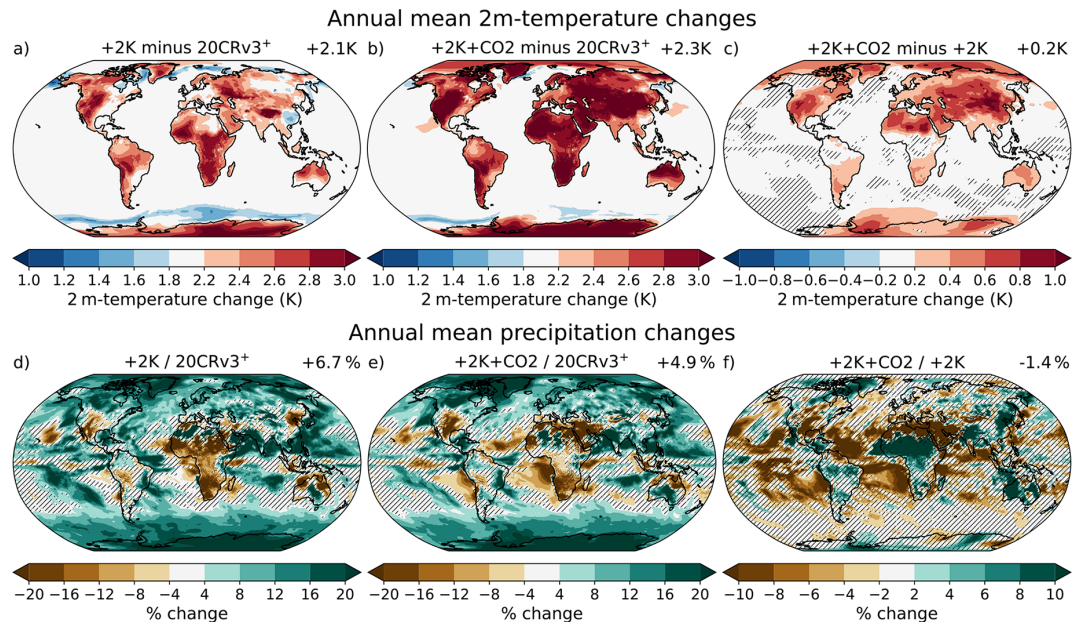
Figure 4. Annual-mean changes in 2 m-temperature (a–c) and precipitation (d–f) between the reanalysis experiments. Changes are shown as differences between experiments for temperature, and as percentage changes between experiments for precipitation. The value at the top right of each plot is the global (area-weighted) average of the changes at each gridpoint (note that this is different to the changes in the global-mean shown in Fig. 3). Hatching obscures non-significant changes at the 5 % level using a two-tailed Student’s t test. The colour bar in panels (a)–(b) is centred on a change of +2 K as this is the perturbation applied to the SSTs.
