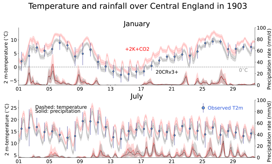
Figure 2. Time series of 3-hourly 2 m-temperature (dotted line) and precipitation rate (solid line) averaged over central England (3–0° W, 51.5–54.0° N, see boxed region in Fig. 8). The 20CRv3 + experiment is in black and the +2 K + CO 2 experiment is in red (see Fig. S1 in the Supplement for the +2 K experiment). Lines show the ensemble-means and shading denotes the 10 %–90 % range across the ensemble. Blue markers show daily-mean temperatures from the Central England Temperature (CET) series (Legg et al., 2025), plotted at 09:00 UTC each day. Vertical bars on each marker indicate the CET daily maximum and minimum temperatures. The grey dashed line in the top panel indicates the air frost threshold (0 °C).
