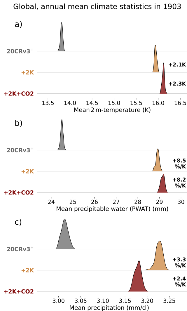
Figure 3. Globally and annually averaged 2 m-temperature (a), total-column precipitable water (PWAT) (b), and precipitation rate (c) in the reanalysis experiments. Curves show the density of values across the 80 ensemble members in each experiment.
