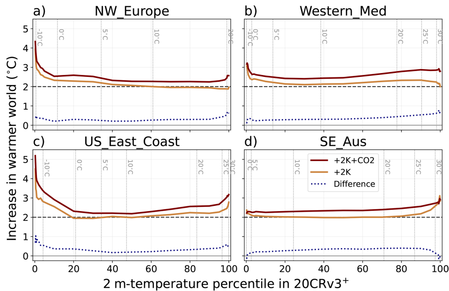
Figure 5. Change in ensemble-mean, daily-mean 2 m-temperature in the warmer world experiments versus 20CRv3 + , as a function of temperature percentile in 20CRv3 + . The pairwise difference between experiments is calculated for every (lat, lon, day) pair and is then binned according to the temperature value of that (lat, lon, day) in 20CRv3 + . Solid lines show the mean difference in each bin. The blue dotted line shows the pairwise difference between the +2 K + CO 2 and +2 K experiments (again binned according to 20CRv3 + temperature). Only land gridcells are used. The horizontal dashed line indicates a change of +2 °C and the vertical dotted lines show absolute temperatures in 20CRv3 + .
