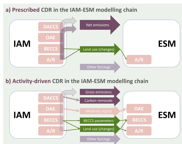
Figure 1. Schematic of prescribed (a) and activity-driven (b) CDR in the IAM-ESM modelling chain. Panel (a) depicts the current state-of-the-art, which has been used for CMIP5 and 6, and is planned for CMIP7. Panel (b) depicts activity-driven CDR as discussed in this paper.
