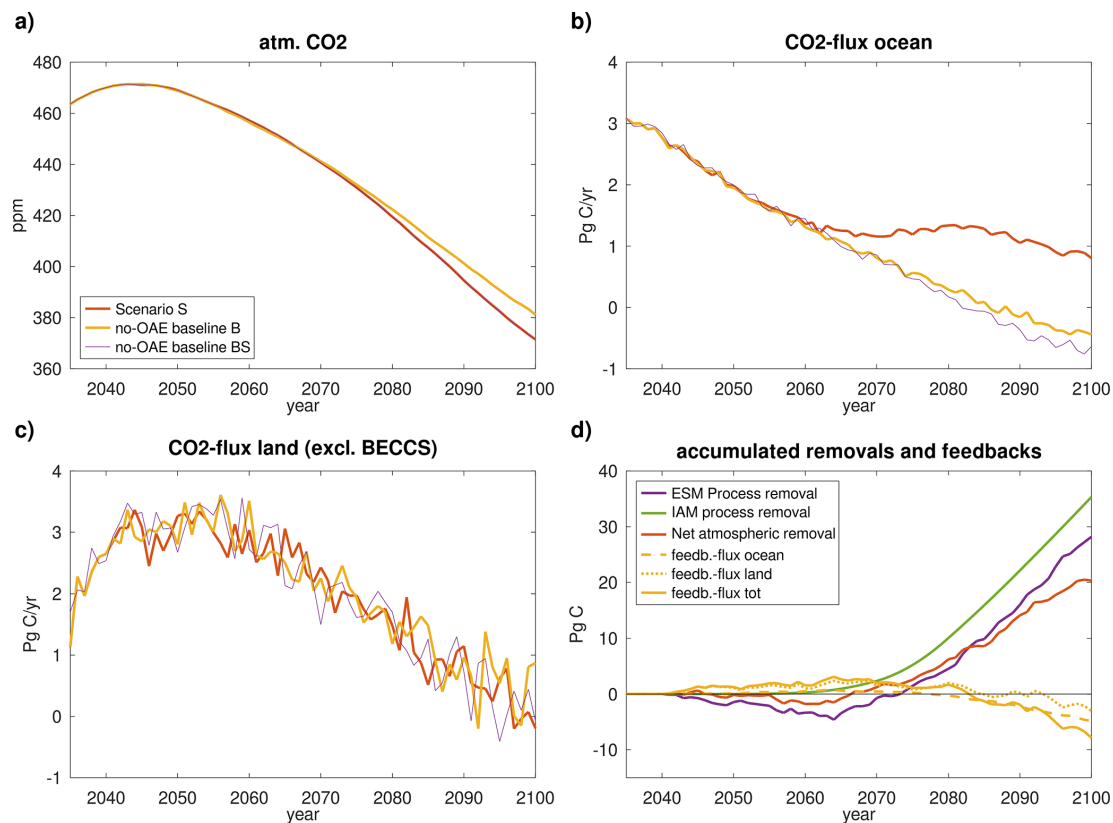
Figure 3. Estimating the net atmospheric and process carbon removals of OAE deployment in a deep mitigation scenario using the two no-CDR baselines B and B S : Atmospheric CO 2 concentration (a), air-sea (b), and air-land (c) CO 2 fluxes in the emission-driven scenario S (red lines), the emission-driven no-CDR baseline B (yellow lines), and the concentration-driven no-CDR baseline B S (atmospheric CO 2 concentrations from S prescribed, thin purple lines). The difference between the yellow and purple lines in panels (b) and (c) is used to derive the feedback contributions according to Eqs. (11) and (12), which is shown by the yellow lines in panel (d). Panel (d) shows the accumulated net atmospheric and process carbon removals due to OAE as well as the accumulated feedback fluxes. The process carbon removal estimated by the IAM is also shown for comparison (line styles and colors as indicated in the legend in panel d).
