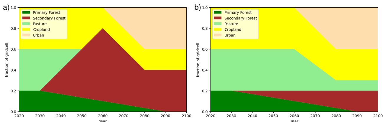
Figure 2. Schematic of a grid-cell undergoing A/R (a) and the proposed strategy for ex-post adjustments (b), where land-use transitions for A/R are “frozen”. In this example forest area is reduced towards the end of the original A/R scenario, which is reflected by transitions of the “frozen” land use towards the land use that replaces the forest in the original scenario.
