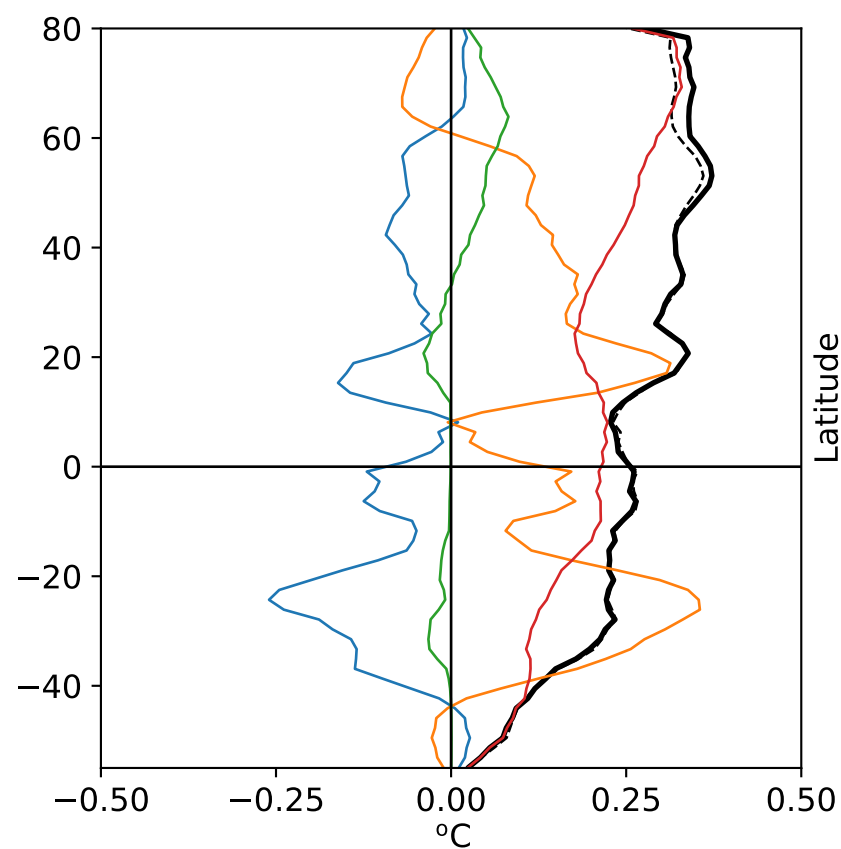
Dynamic Ocean Simulation
