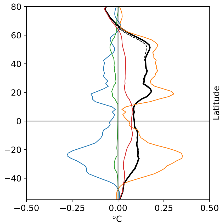
Prescribed SST Simulation
