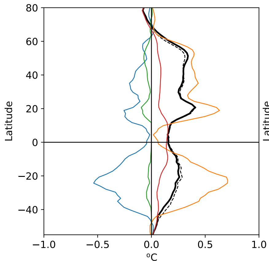
Prescribed SST Simulation
