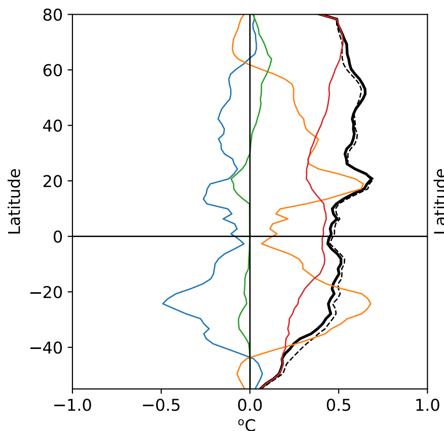
Dynamic Ocean Simulation
