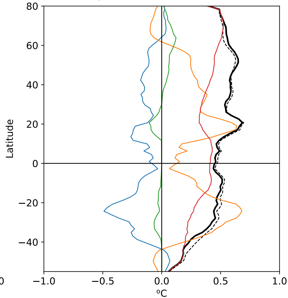
Dynamic Ocean Simulation
