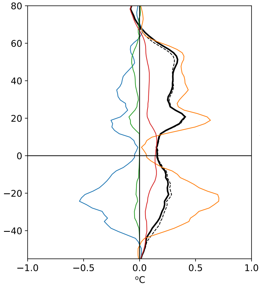
Prescribed SST Simulation
