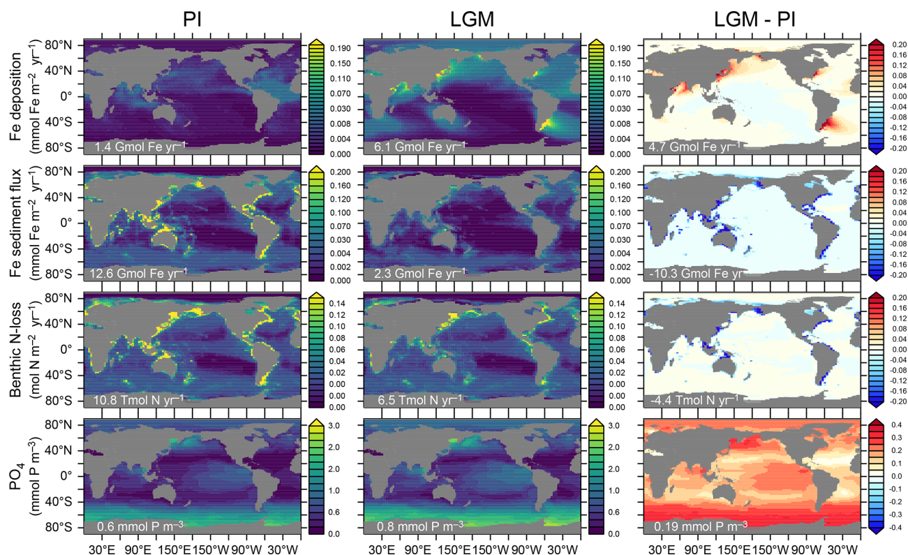
Figure 2. Fe deposition and sedimentary fluxes, benthic denitrification (benthic N-loss), and surface \text{PO}_4^{3-} in the PIallbgc and LGM biogeochemical configurations and their differences. PI results are the means of 20 simulations in PIctl_Pllallbgc, and LGM Fe deposition, Fe sedimentary flux, benthic denitrification, and surface \text{PO}_4^{3-} are from PIctl_LGMFedep, PIctl_LGMFesed, PIctl_LGMBdeni, and PIctl_LGMPO 4 simulation means. Values on the bottom left of each panel indicate the global annual Fe and N fluxes or \text{PO}_4^{3-} concentration.
