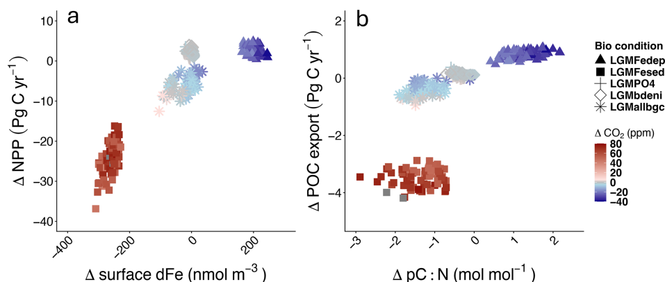
Figure 7. Differences in (a) NPP and surface dFe and (b) POC export and pC : N with respect to default biogeochemical conditions (Plallbgc). Color represents atmospheric p\text{CO}_2 and symbols indicate the different biogeochemical configurations. The cluster of points with little deviation from *_Plallbgc simulations is from *_LGMPO4 and *_LGMbdeni simulations.
