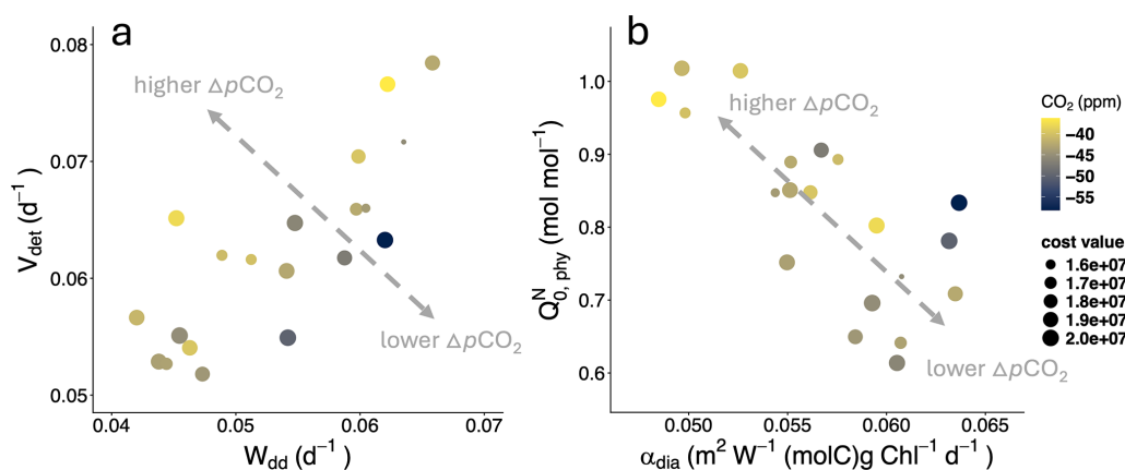
Figure 9. Effects of parameter pairs on the \Delta p\text{CO}_2 between Pictl_Pfallbgc and LGMatmctl_LGMallbgc. (a) \nu_{\text{det}} and w_{\text{dd}} and (b) \alpha_{\text{dia}} and Q_{0,\text{phy}}^{\text{N}} are the most positively and negatively correlated pairs in the 19 parameters, respectively.
