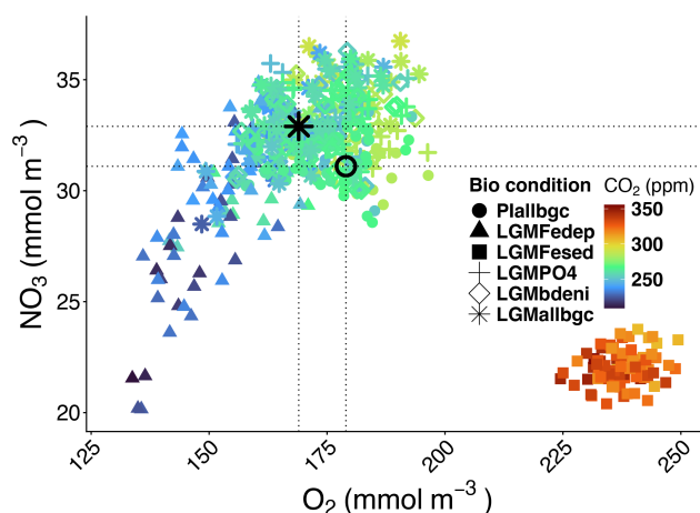
Figure 8. Globally-averaged NO_3^- vs. O_2 in the 480 simulations. Color represents atmospheric pCO_2 and symbols indicate the different biogeochemical configurations. The black open circle and asterisk indicate mean NO_3^- and O_2 in Pictl_PIallbgc and LGMatmctl_LGMallbgc simulations, respectively. The cluster of points with high pCO_2 and low NO_3^- is from *_LGMFesed simulations.
