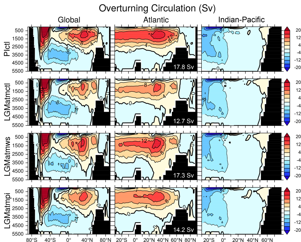
Figure 6. Meridional overturning streamfunction in the Global, Atlantic, and Indian-Pacific Oceans for P1ctl, LGMatmctl, LGMatmws, and LGMatmpi, all combined with the P1allbgc biogeochemical configuration. Results are ensemble means over the 20 simulations in each of the configurations. Values in white indicate the strength of maximum AMOC at 26.5°N under each condition.
