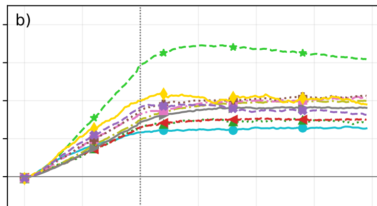
Mid-lat esm-flat10-zec
