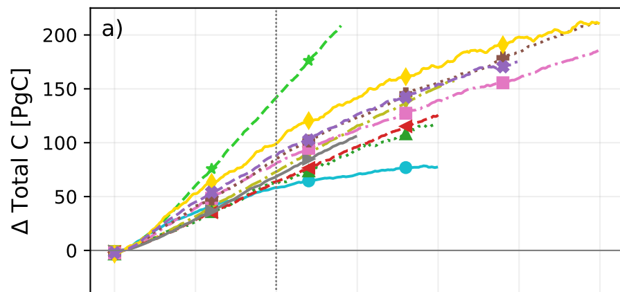
Mid-lat esm-flat10
