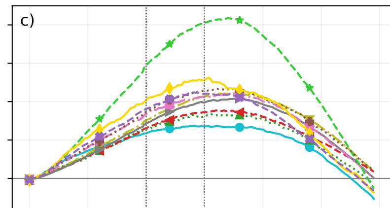
Mid-lat esm-flat10-cdr
