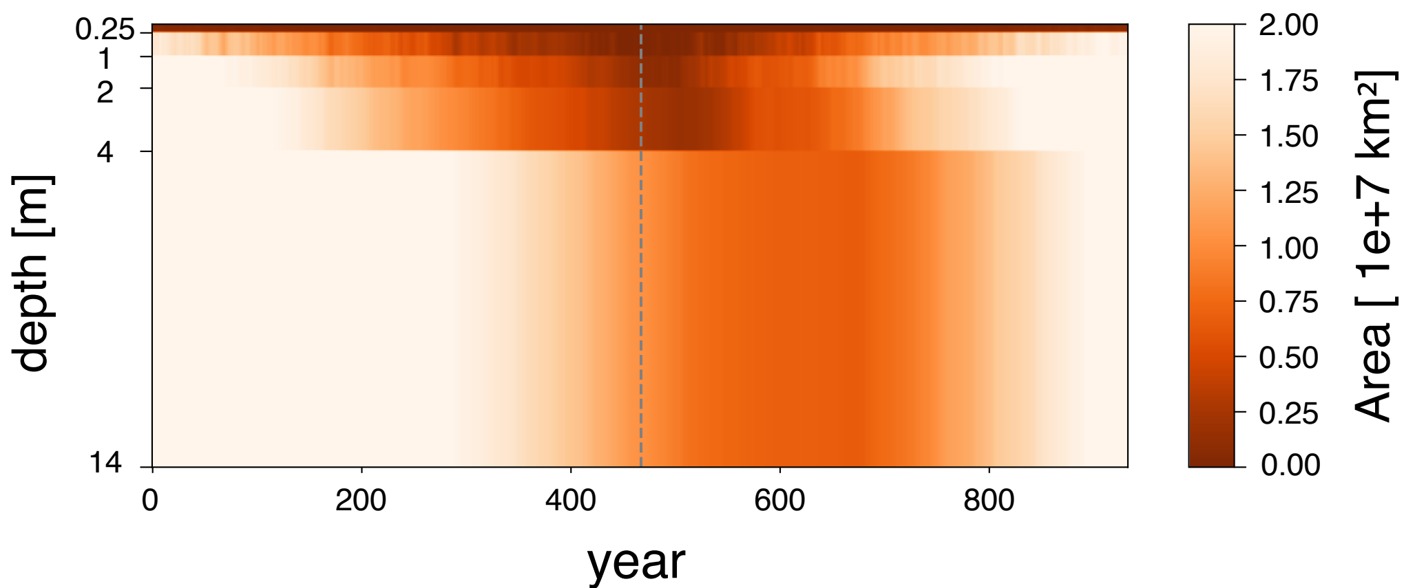
Permafrost Area by depth
