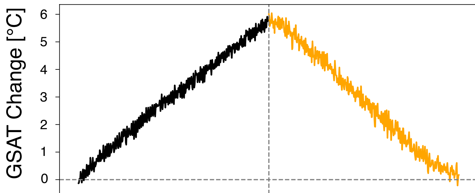
GSAT Change
