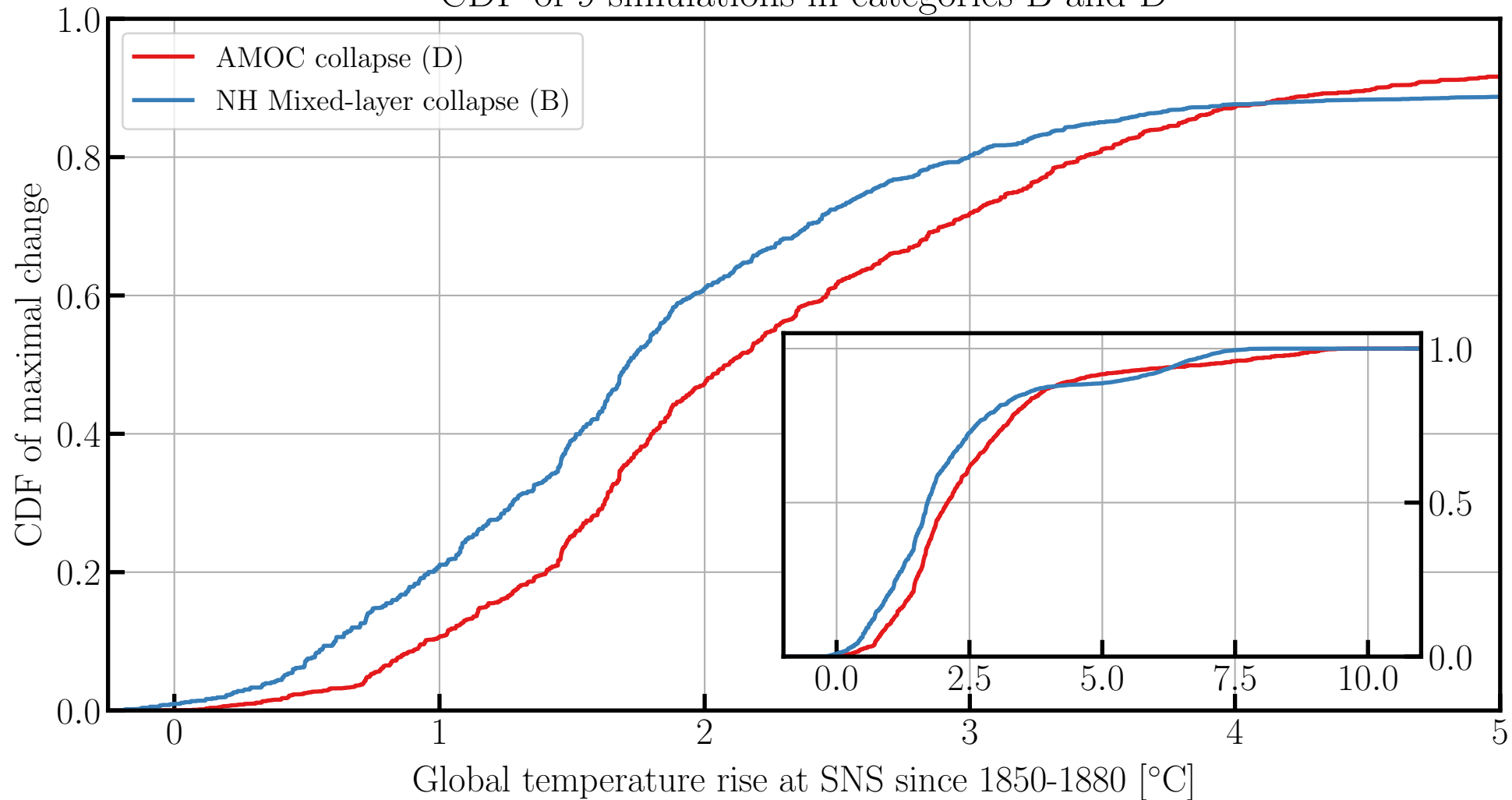
CDF of 9 simulations in categories B and D
