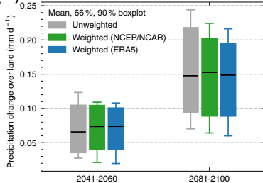
(b) SSP3-7.0 projections relative to 1995-2014
