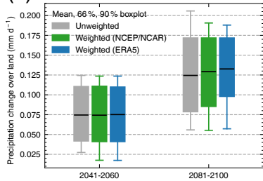
(c) SSP2-4.5 projections relative to 1995-2014
