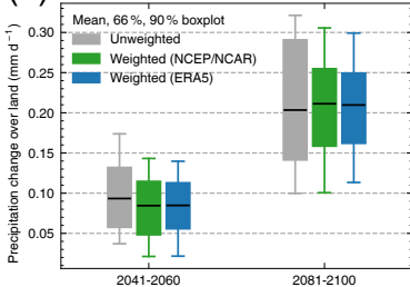
(a) SSP5-8.5 projections relative to 1995-2014
