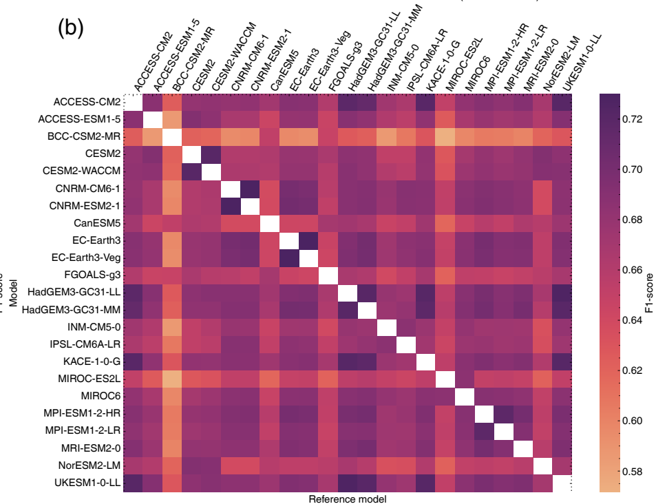
Inter-similarities of the climate models' causal networks (ERA5 modes)
