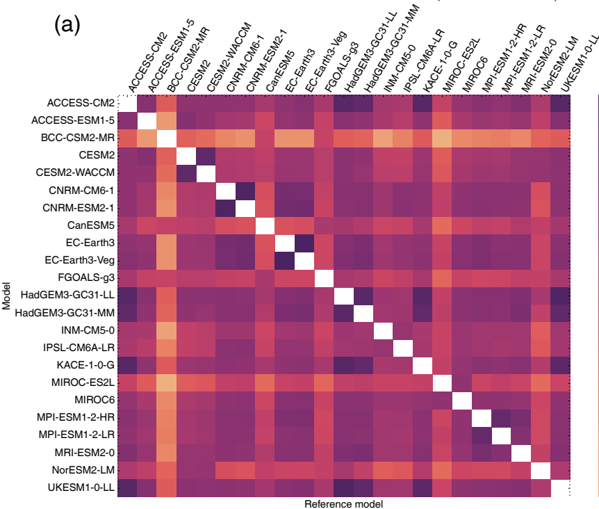
Inter-similarities of the climate models' causal networks (NCEP/NCAR modes)
