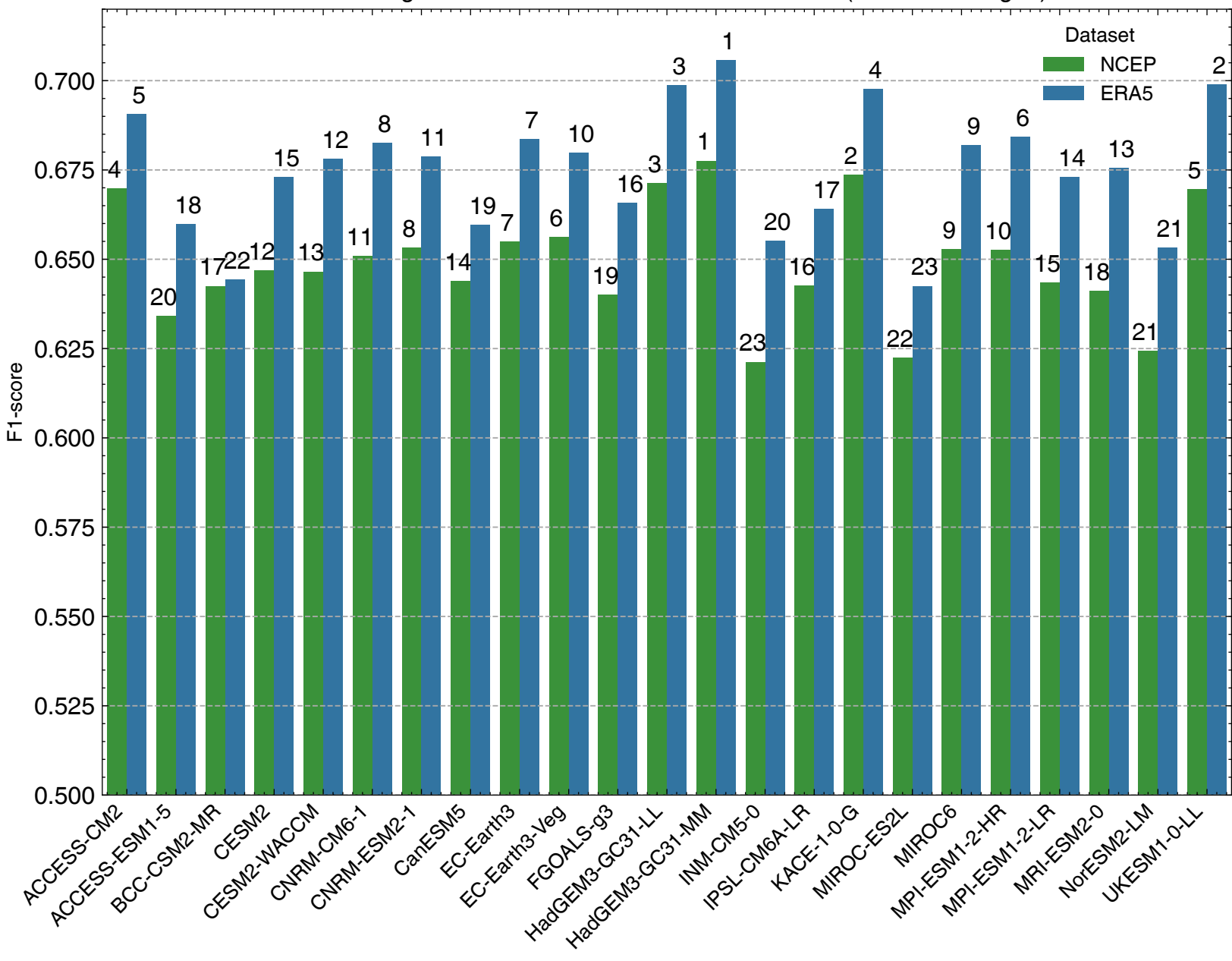
F1-score against NCEP/NCAR and ERA5 networks (season-averaged)
