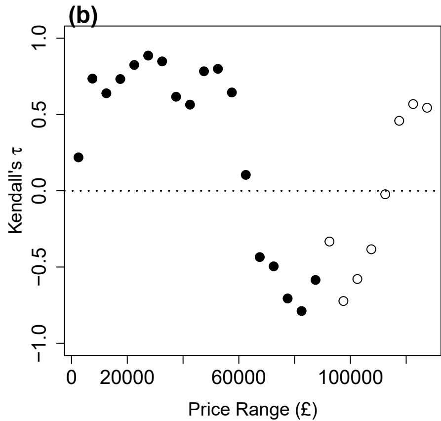
Variance
