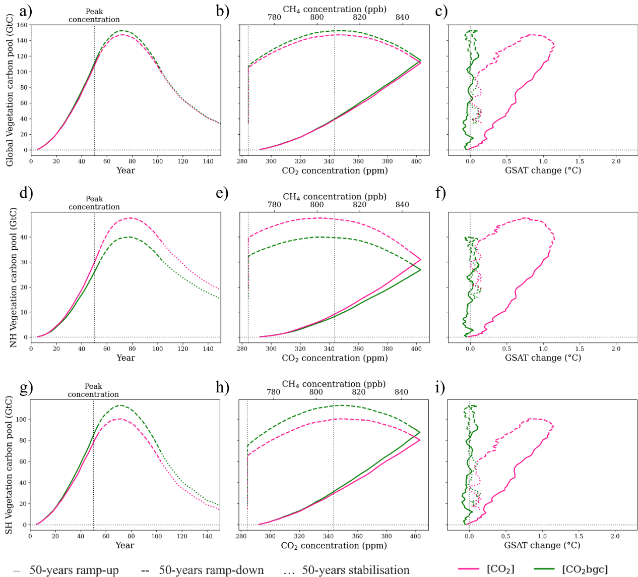
Figure S10. (a–c) Global, (d–f), northern high-latitude ( >30^{\circ} N) and (g–i) subtropical and southern ( <30^{\circ} N) changes in vegetation carbon pool (GtC), as a function of (a, d, g) time (year), (b, e, h) \text{CO}_2 concentration (ppm) / \text{CH}_4 concentration (ppb, only for [non \text{CO}_2 ]) and (c, f, i) GSAT ( ^{\circ}\text{C} ) under selected scenarios.
