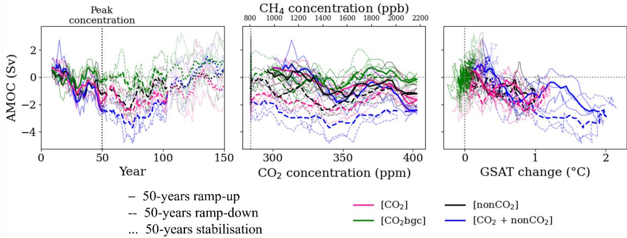
20 Figure S1. (a) Comparison of the Atlantic Meridional Overturning Circulation (AMOC) time evolution in the IPSL-CM6A-LR idealised experiments relative to the initial date in the pre-industrial control simulation. Time evolution of the 5-year moving average AMOC (Sv) from the piControl simulation (grey) and from the idealised experiments. (b) AMOC as a function of time (year), CO 2 concentration (ppm) / CH 4 concentration (ppb, only for [nonCO 2 ]), and GSAT (°C) under selected scenarios. Thick lines indicate the ensemble means and thin lines correspond to three ensemble members.
