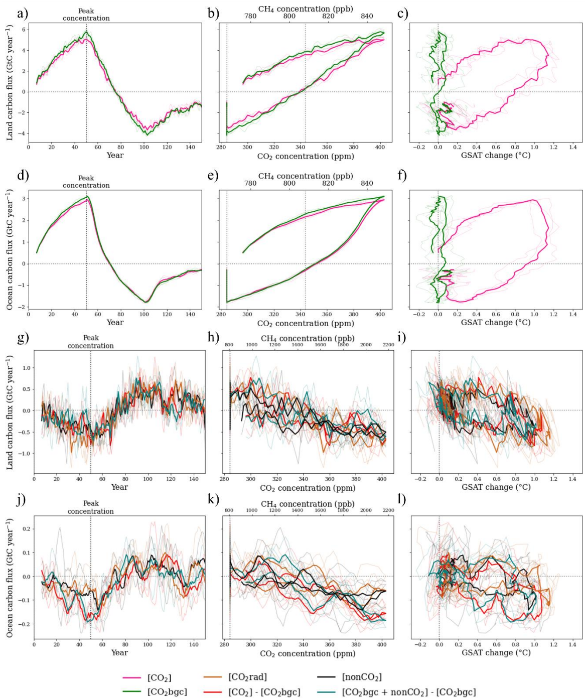
Figure S6. Global (a–c, g–i) land and (d–f, j–l) ocean carbon flux, positive sink to the land/ocean (GtC year -1 ) as a function of (a, d, g, j) time (year), (b, e, h, k) CO 2 concentration (ppm) / CH 4 concentration (ppb, only for [nonCO 2 ]) and (c, f, i, l) GSAT (°C) under selected scenarios.
