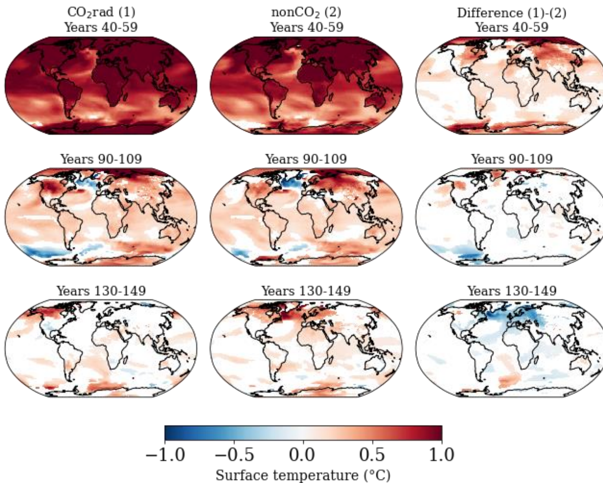
40 Figure S4. Spatial variation of three-member-ensemble mean changes in surface temperature (°C) averaged over 20 years at the end of (first rows) ramp-up, (middle rows) ramp-down, and (bottom rows) stabilisation phases in the [CO 2 rad] and [nonCO 2 ] experiment. We draw only significantly different grids using three ensemble members ( p < 0.1 based on t test, N=60).
