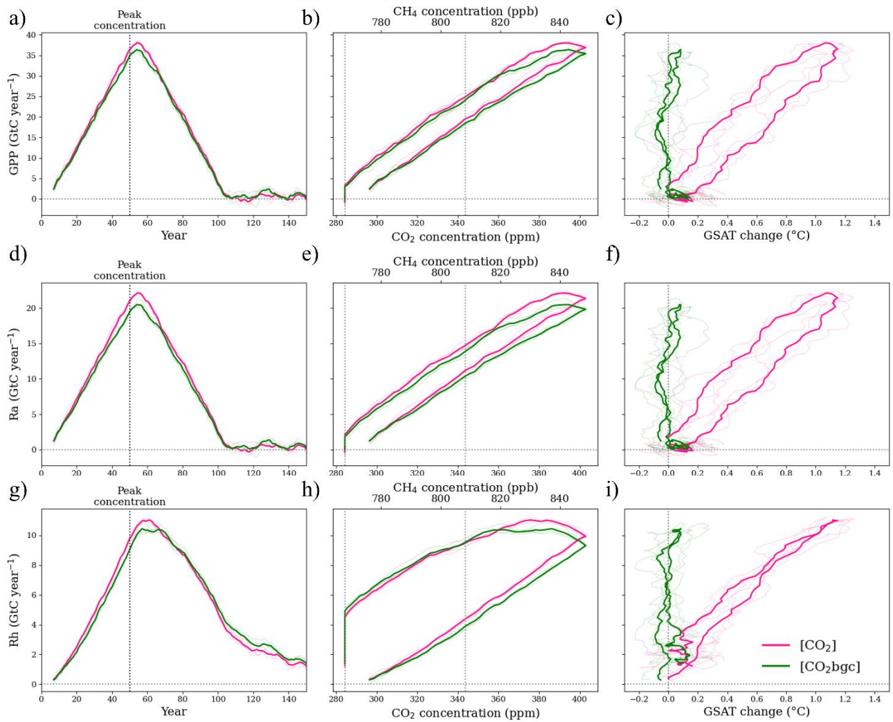
Figure S7. Global (a–c) GPP, (d–f) Ra and (g–i) Rh (GtC year -1 ) as a function of (a, d, g) time (year), (b, e, h) CO 2 concentration (ppm) / CH 4 concentration (ppb, only for [nonCO 2 ]) and (c, f, i) GSAT (°C) under selected scenarios.
