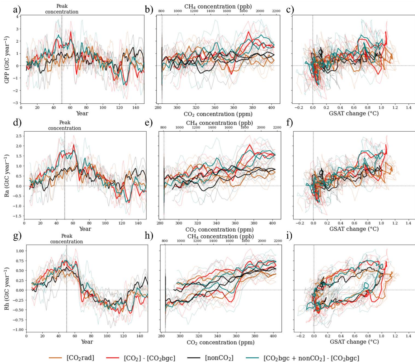
Figure S7 (continued). Global (a–c) GPP, (d–f) Ra and (g–i) Rh (GtC year -1 ) as a function of (a, d, g) time (year), (b, e, h) CO 2 concentration (ppm) / CH 4 concentration (ppb, only for [nonCO 2 ]) and (c, f, i) GSAT (°C) under selected scenarios.
