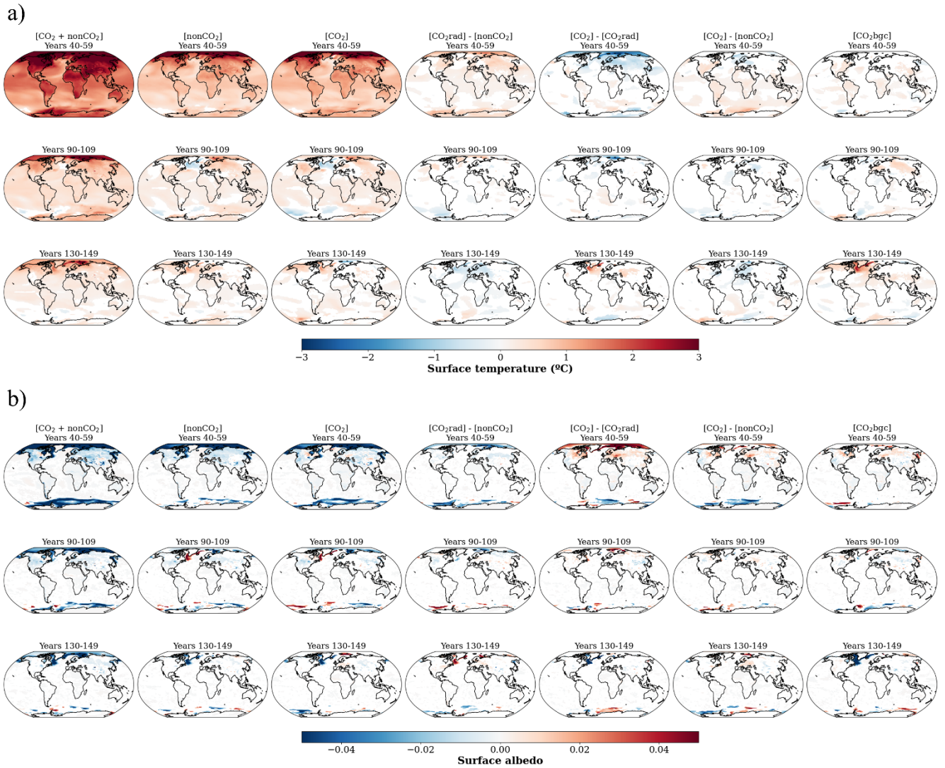
35 Figure S3. Spatial variation of three-member-ensemble mean changes in (a) surface temperature (°C) and (b) surface albedo averaged over 20 years at the end of (first rows) ramp-up, (middle rows) ramp-down, and (bottom rows) stabilisation phases relative to piControl under selected scenarios. We draw only grids significantly different from piControl ( p < 0.1 based on t test, N=60 ) and between [CO_2] , [CO_2rad] and [nonCO_2] experiments using three ensemble members ( p < 0.1 based on t test, N=60 ).
