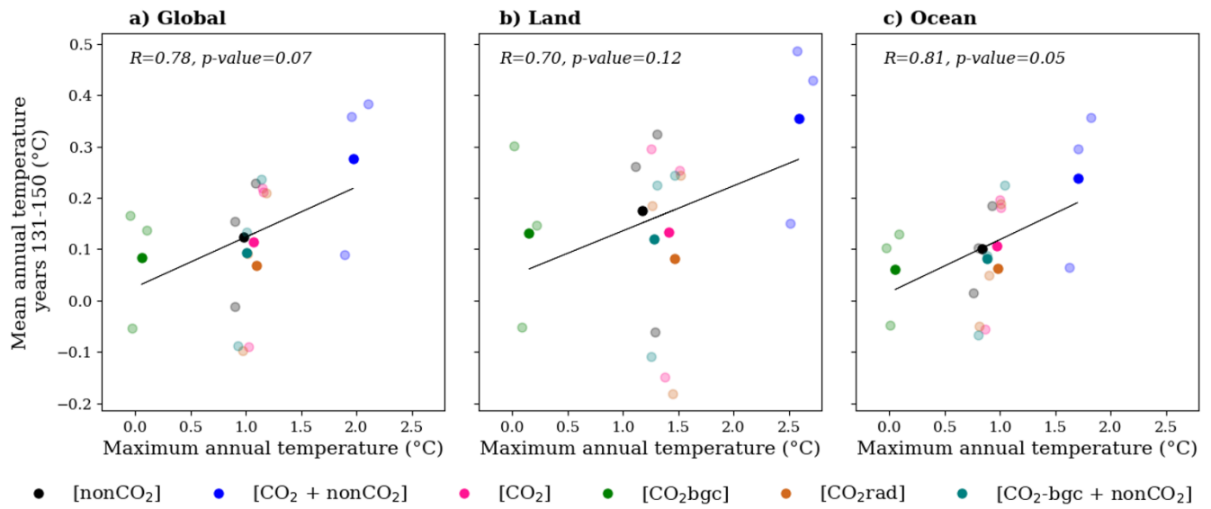
Figure S2. (a) Global, (b) land and (c) ocean mean annual surface averaged over the last 20 years of each experiment plotted against corresponding maximum annual temperature for each experiment and each ensemble member (transparent dots) and ensemble means (solid dots). The correlation coefficients are calculated for ensemble means.
