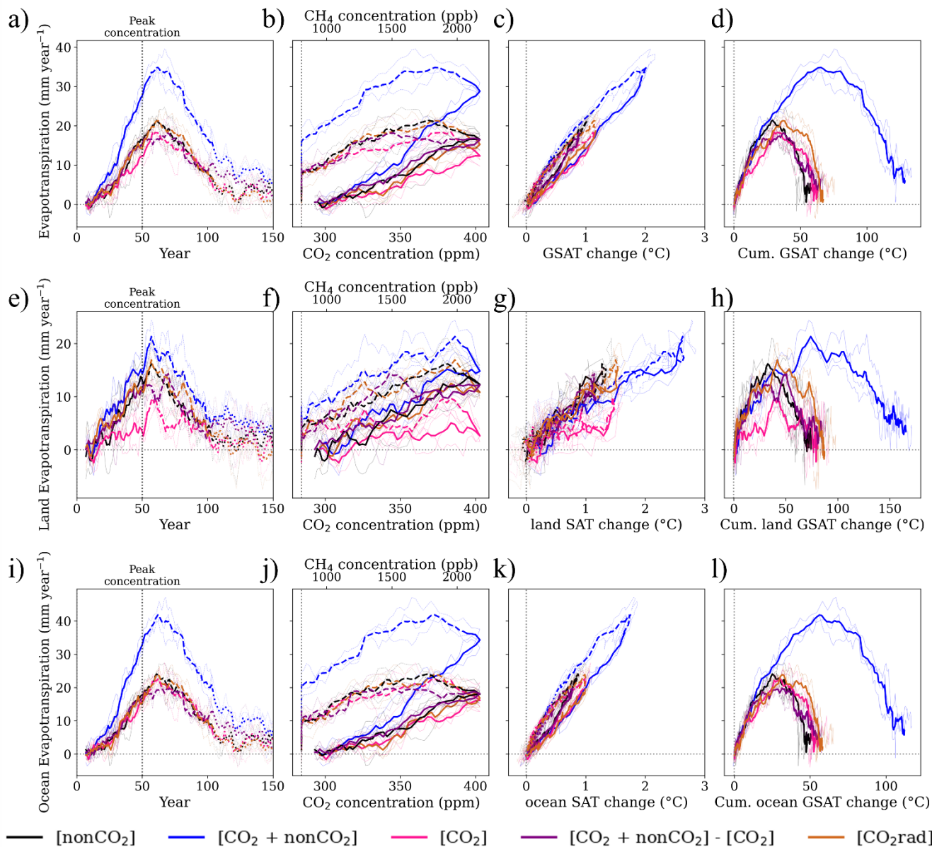
45 Figure S5. (a–d) Global, (e–h) land and (i–l) ocean annually-averaged changes in evapotranspiration (mm year -1 ) as a function of (a, e, i) time (year), (b, f, j) CO 2 concentration (ppm) / CH 4 concentration (ppb, only for [nonCO 2 ]), (c, g, k) GSAT (°C) and (d, h, l) cumulative GSAT (°C).
