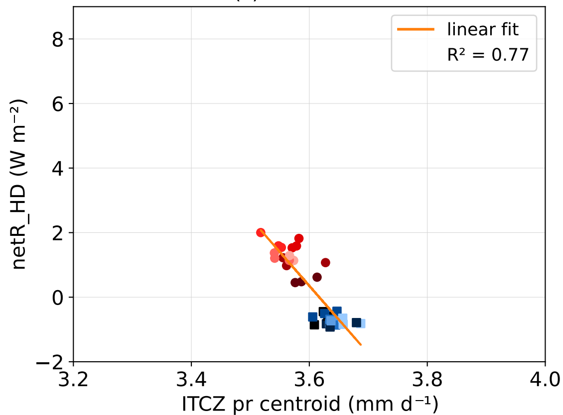
(c) MRI-ESM2-0
