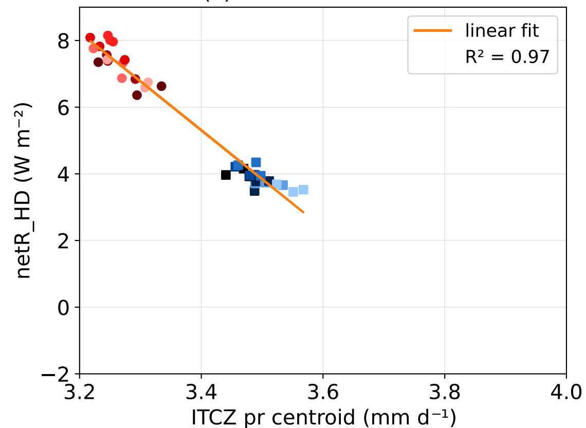
(b) EC-Earth3-AerChem
