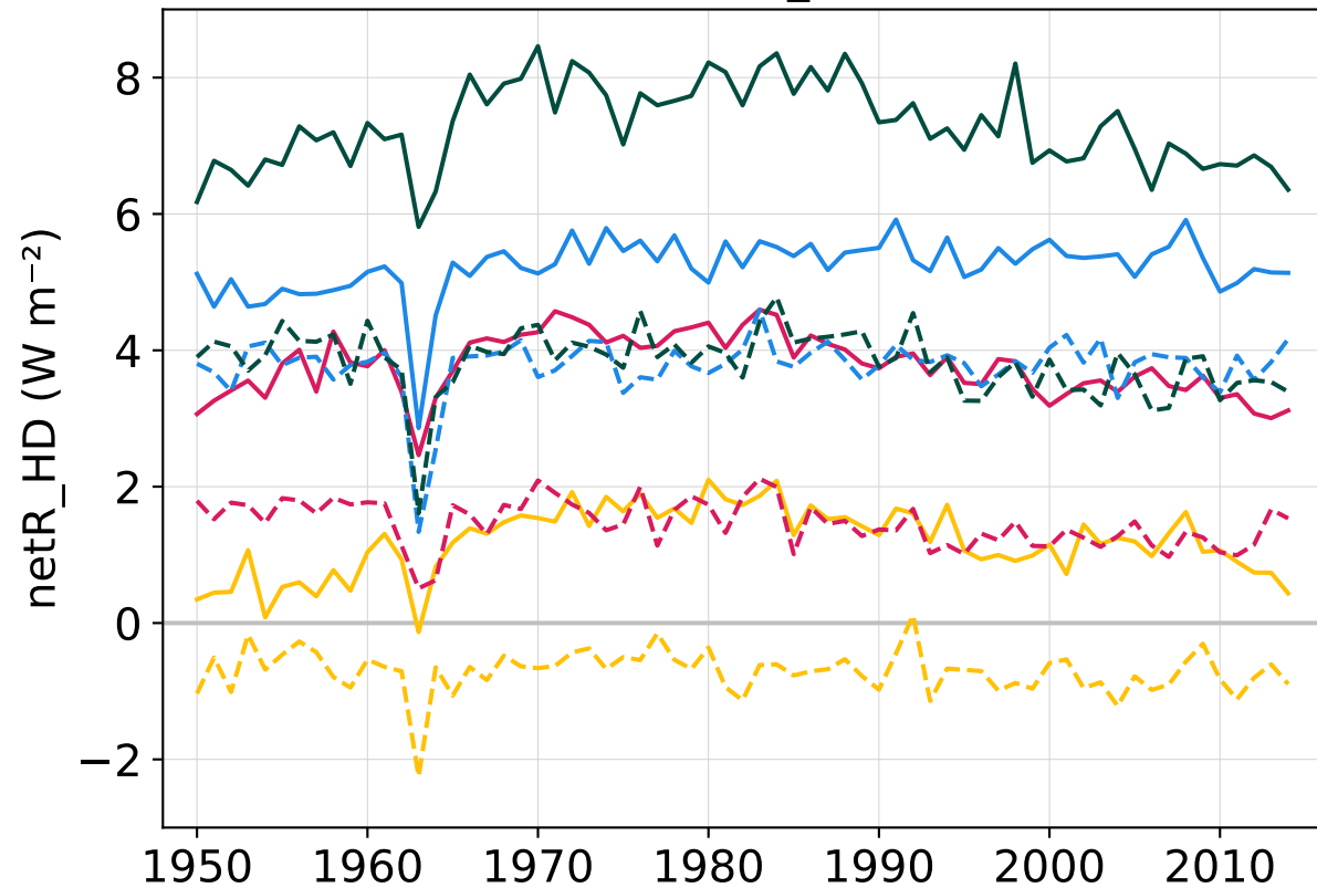
(a) netR_HD
