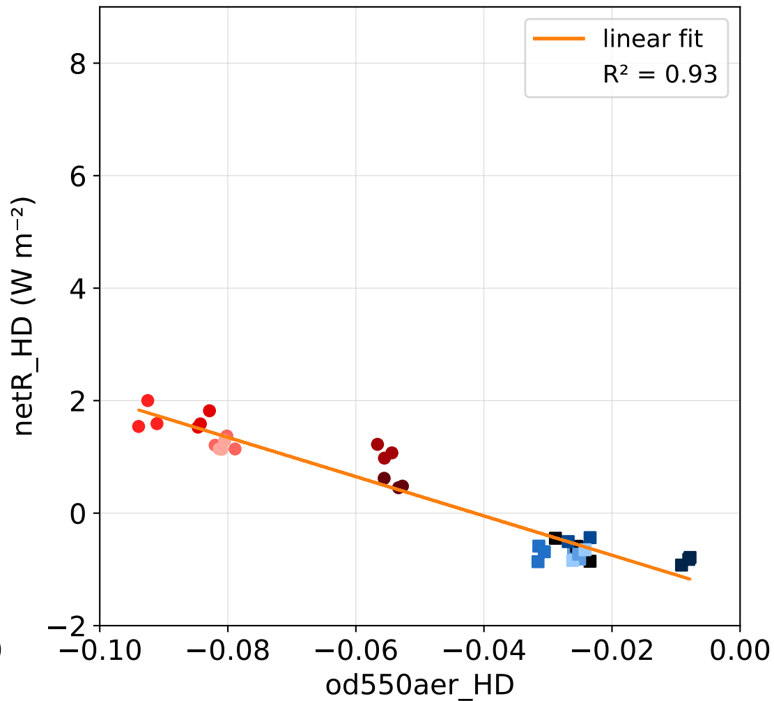
(b) MRI-ESM2-0
