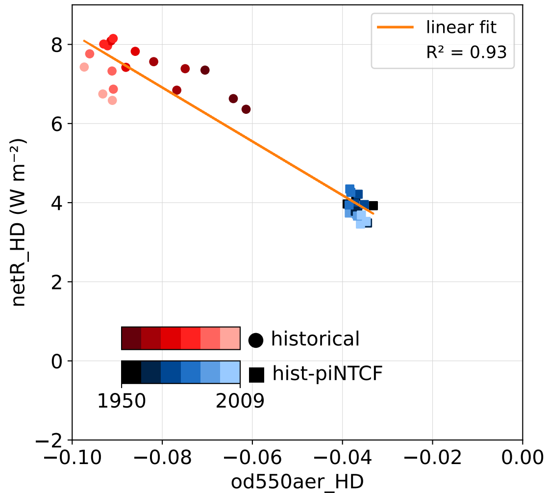
(a) EC-Earth3-AerChem
