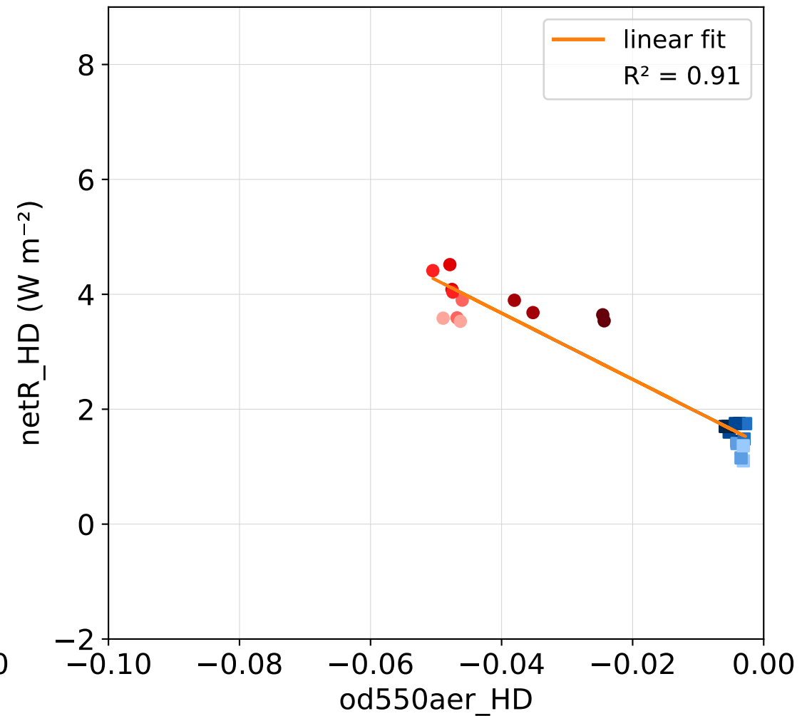
(c) UKESM1-0-LL
