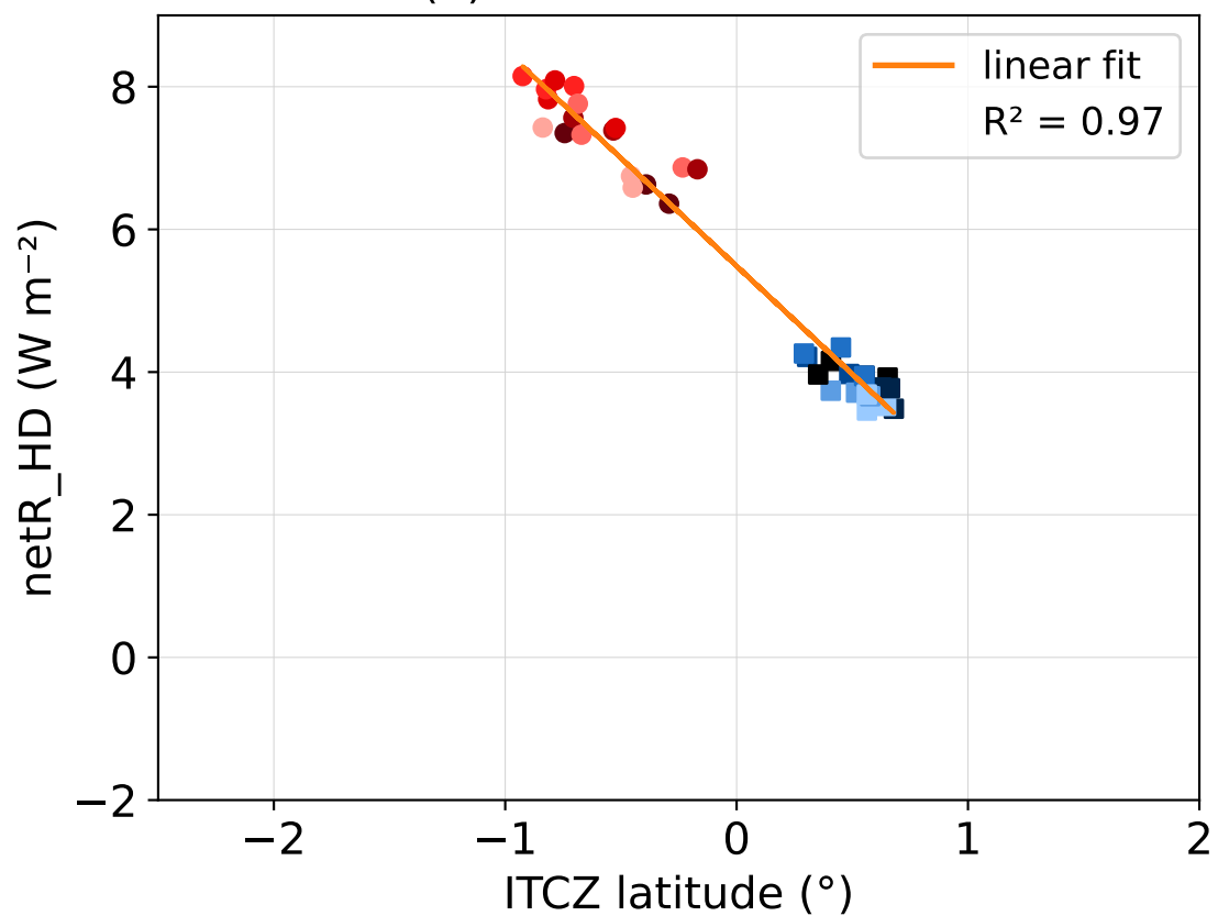
(b) EC-Earth3-AerChem
