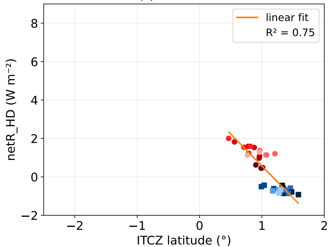
(c) MRI-ESM2-0
