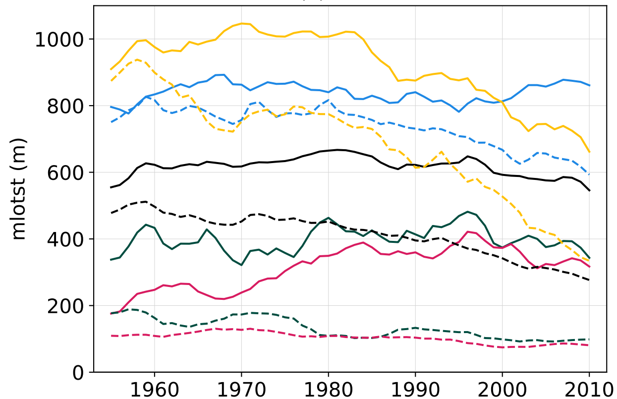
(a) mlotst
