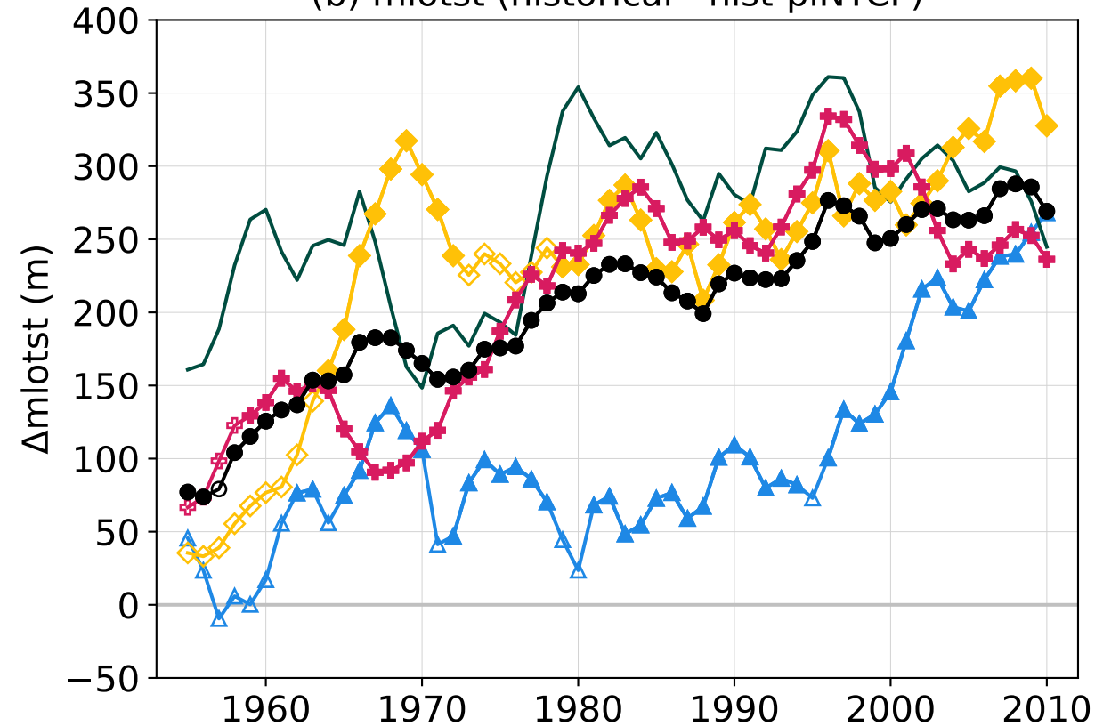
(b) mlotst (historical - hist-piNTCF)
